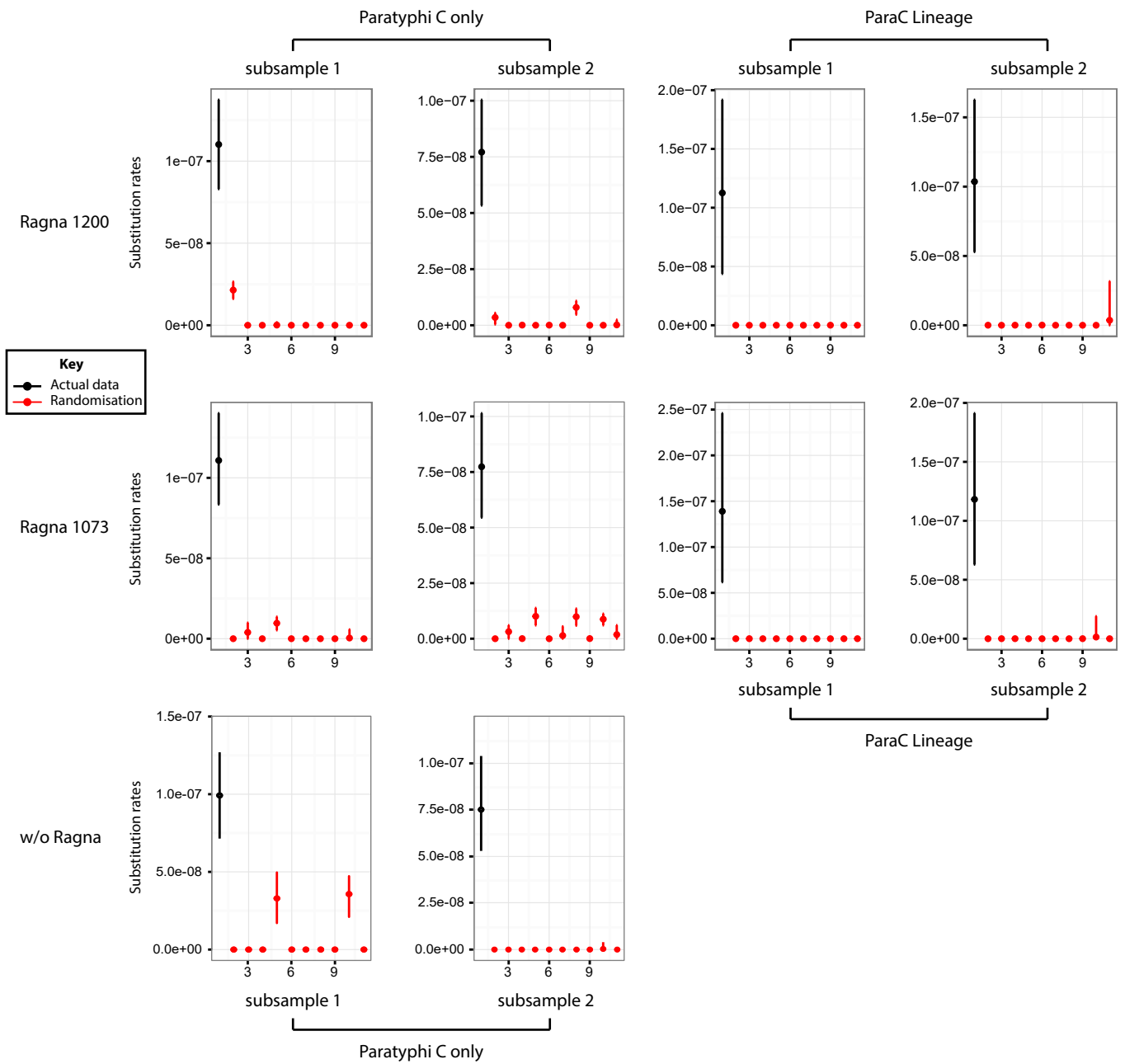
Date estimation 1. Date randomization tests for the temporal signal in multiple replicate data sets that were analysed by BEAST (Table S4; Date estimation 3). Solid circles represent mean estimates of substitution rates, and errors bars show their 95% credible intervals. Black symbols were estimated with real data and red symbols were obtained from 10 randomizations of dates per data set.
