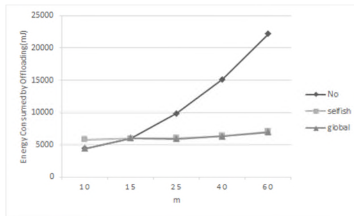
Figure10. The energy consumption of the native App, application developed by SOM and application by GOM
