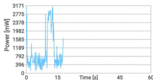
Figure 9. Testing the power consumption with the Trepn Profiler
