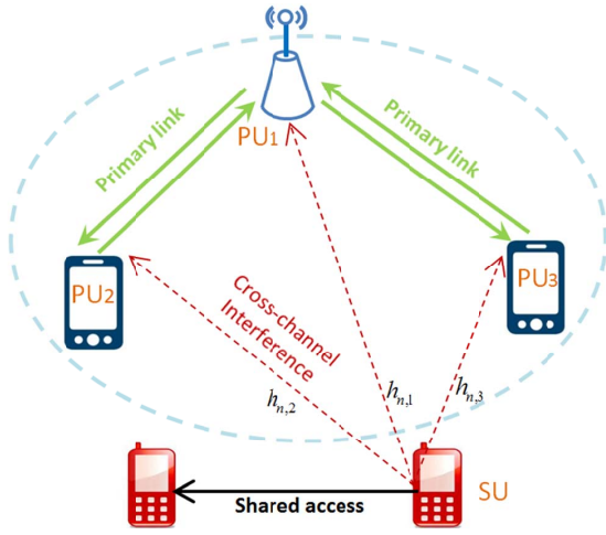
Fig. 1. Shared access and transmission between heterogeneous D2D devices and an indoor TDD small-cell network.
