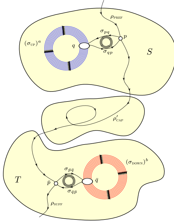
Figure 2: The construction of \rho'_{\text{CAP}} in the first part of the proof of Claim 5.5. Note that cycles (\sigma_{\text{PRE-CONN}})^c and (\sigma_{\text{POST-CONN}})^c are depicted symbolically as small spirals.
