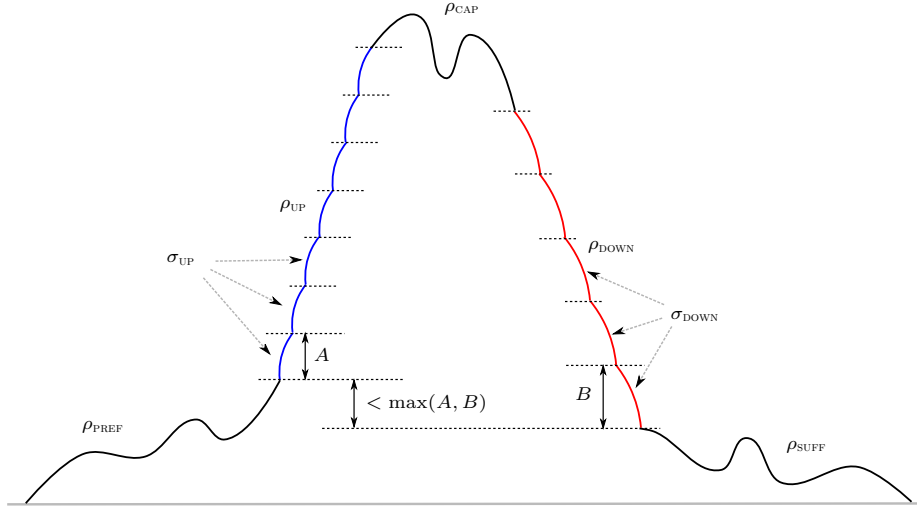
Figure 1: The normal decomposition of an arc together with some notation from the proof of Lemma 5.3.
