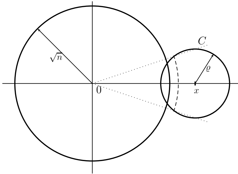
Figure 1. Concentration outside S(0, \sqrt{n}) .
