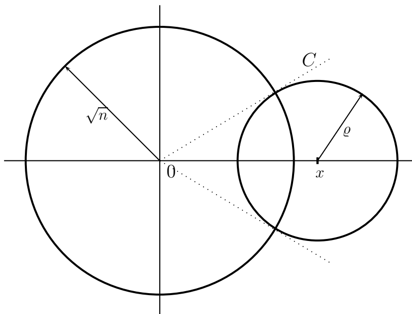
Figure 2. Concentration on S(0, \sqrt{n}) .
