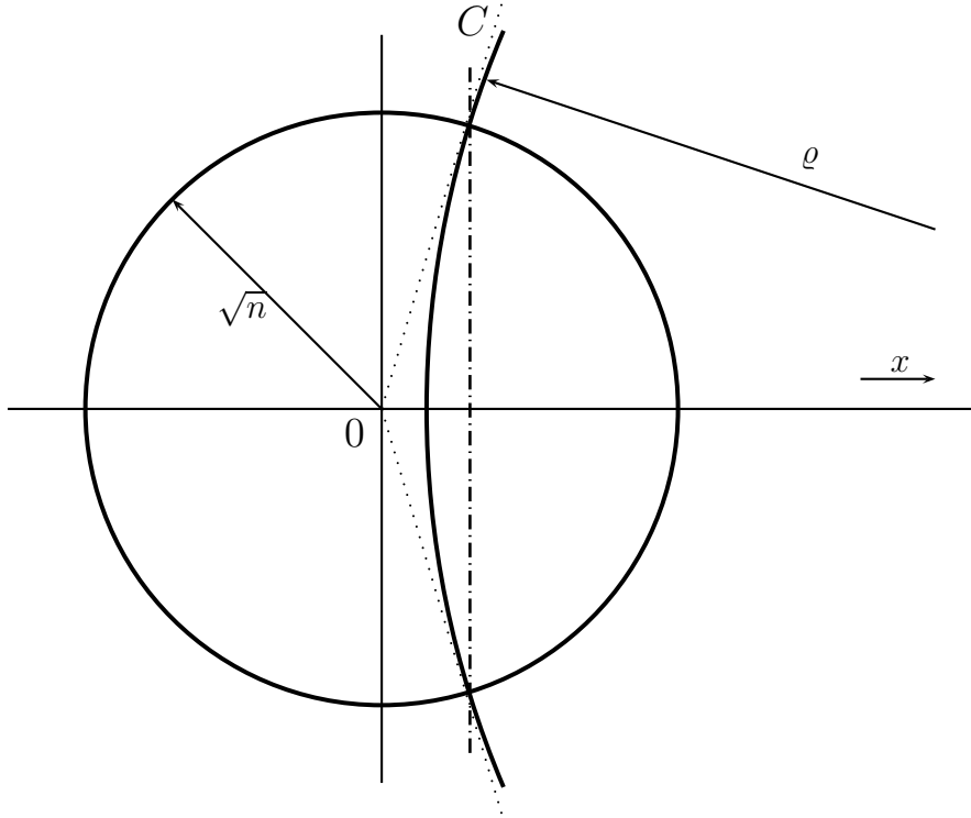
Figure 3. Concentration far from S(0, \sqrt{n}) \cap x^\perp .
