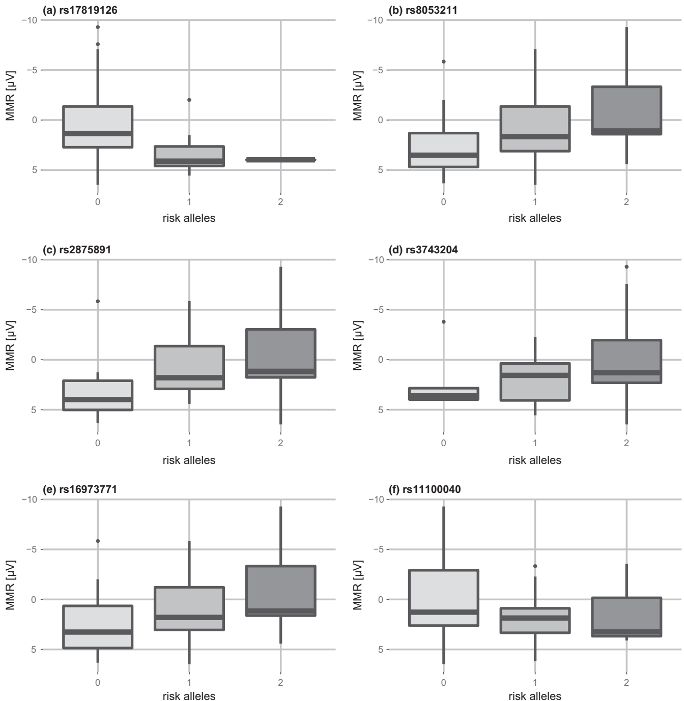
FIGURE 3 Effects of the nominal significant associated single-nucleotide polymorphisms (SNPs) on MMR. Boxplots are shown according to the number of risk alleles of each SNP
