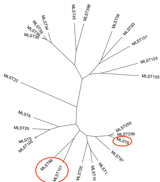
(c) No topology moves using “furthest” ordering.
