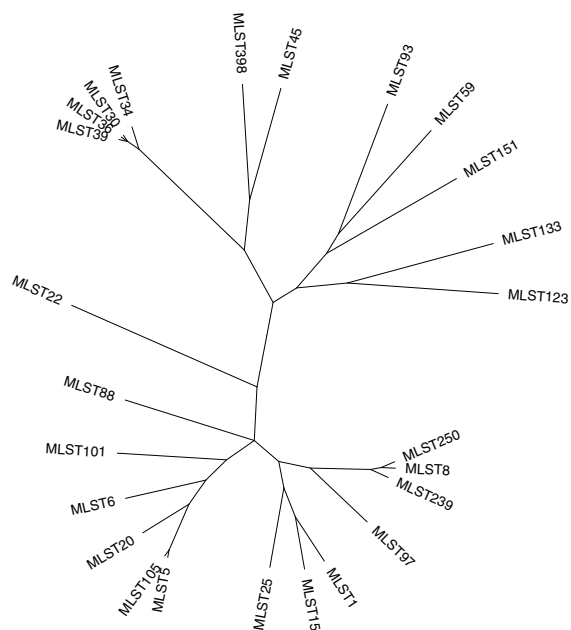
(a) MCMC using 50 million iterations.
