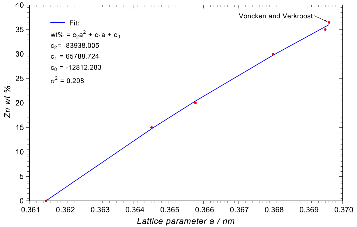
Figure S7: Parabolic fit to data from Rendle (1981) and Voncken & Verkrroost (1997) for Zn wt% as a function of lattice constant. A parabolic rather than linear fit has been used because Vegard's law rarely applies to metallic solid solutions (Suryanarayana & Norton, 1998). Rendle used a similar fit although the curve is not specified.
