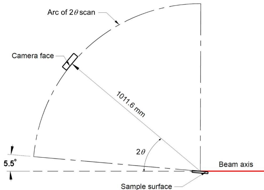
Figure S2: Geometry of SR-XRD measurements
