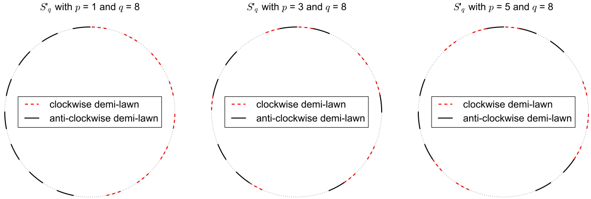
FIG. 2. Sketch of an optimal antipodal lawn S'_q for a rational jump \phi = \pi \frac{p}{q} with odd numerator p = 1 (left), p = 3 (middle), p = 5 (right), and (in all panels) q = 8 . The two demi-lawns are marked by different line styles (black solid lines and red dashed lines).
