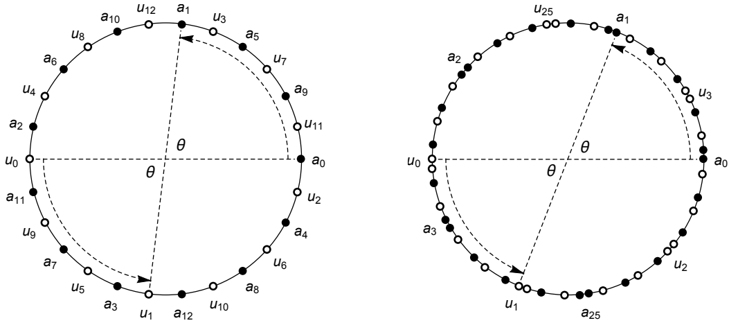
FIG. 3. Construction of modified lawns for rational \phi = p\pi/q and p even, with p = 6 and q = 13 (left panel, Lemma 19) and for irrational \phi/\pi with \phi = 1.2 (right panel, Lemma 20) The caps and cups around the equator are shown as black and white dots respectively.
