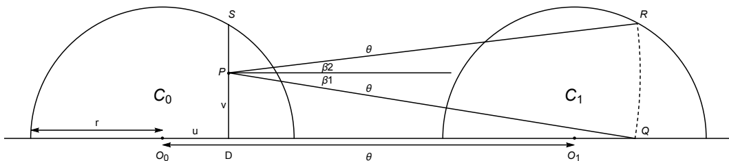
FIG. 5. Jump geometry
