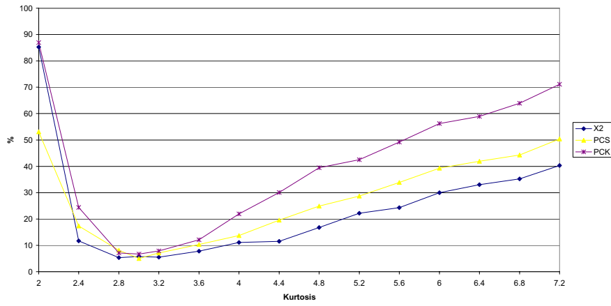
Figure 13: Power for the \chi^2 , PCS and PCK tests for nonequiprobable splits: Ramberg distribution (n=150)
