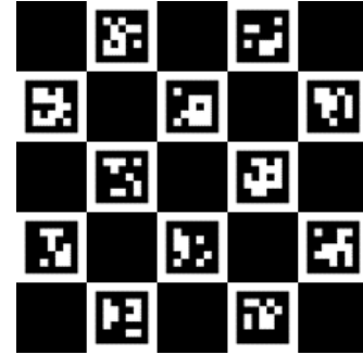
FIGURE 14: CharuCo target [100].
