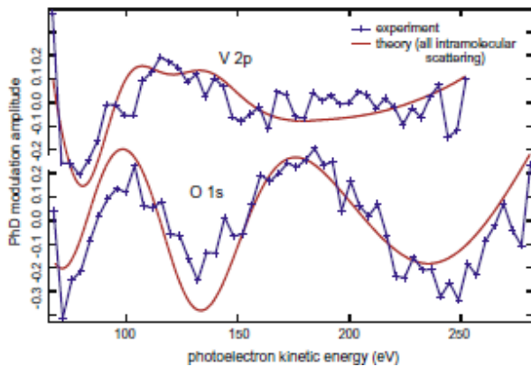
Fig. 4 Comparison of the averaged experimental O 1s PhD and V 2p spectra from VOPc on Au(111) (fig. 2) with the results of multiple-scattering simulations for the structurally-optimised model (with the V=O bond pointing out from the surface) including scattering from all atoms within the molecule. The overall R -factor is 0.29.
