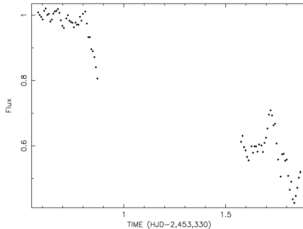
Figure 2. Lightcurve of the continuum light of LMC X-2 where the first night is normalised to unity.
