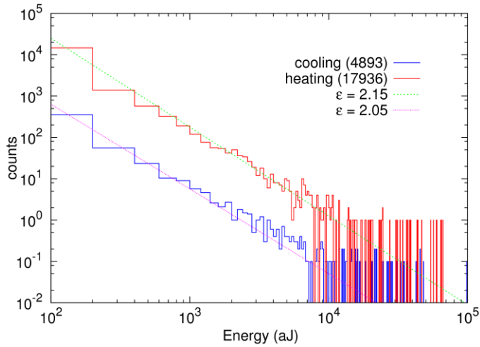
Fig. 9 (Color online) Statistical analysis of the AE observations. Data corresponding to cooling experiments have been shifted one decade downwards in order to clarify the picture.
