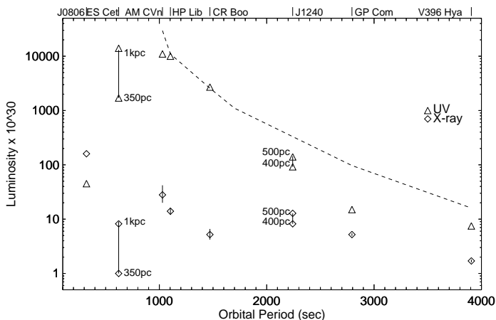
Fig. 4. The (unabsorbed) X-ray and UV luminosities of the AM CVn systems included in this sample. The X-ray luminosities were determined using modelling the X-ray spectrum derived from XMM-Newton data, and the UV luminosities were determined assuming a blackbody of temperature of 30000K. The dotted line is the predicted accretion luminosity – see §7.2 for details.
