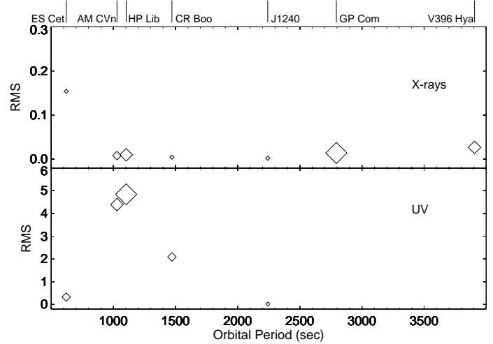
Fig. 1. The rms of the amplitude spectra of the light curves of AM CVn systems in the 0.1-1.0keV X-ray band (top panel) and the UV (bottom panel). The size of the symbol reflects the apparent brightness in that energy. No UV fast mode data were obtained of GP Com and V396 Hya.
