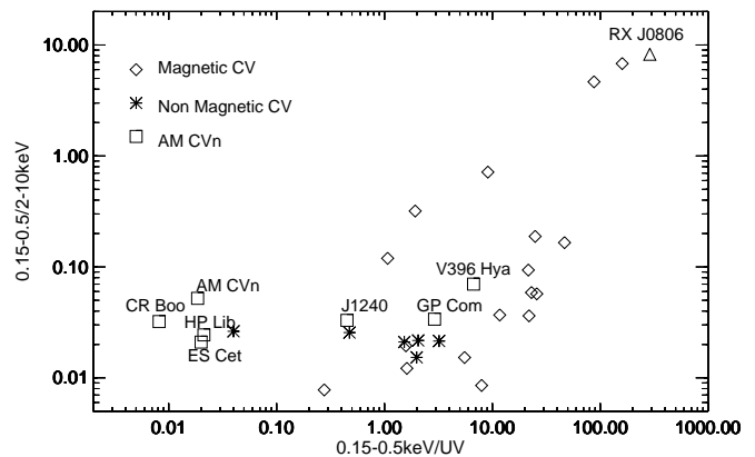
Fig. 3. The colours for the AM CVn systems in this paper; non-magnetic CVs and the strongly magnetic CVs in the 0.15-0.5/2-10keV, 0.15-0.5/UV plane. We also show the colours of the candidate system RX J0806+15. The error on the colours are of a similar size as the symbols.
