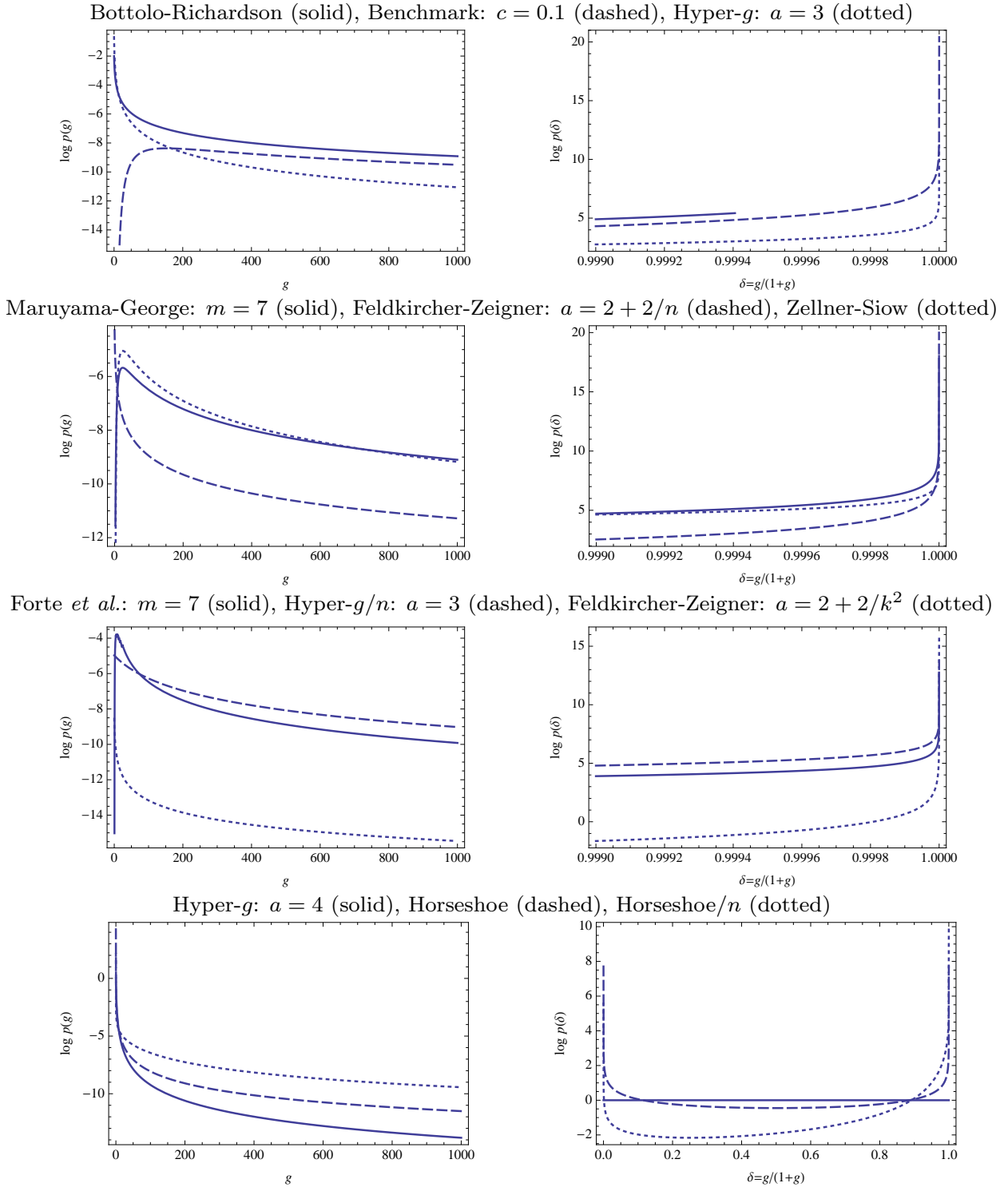
Fig. 2. Priors for g and \delta ( n = 72 , k = 41 )
