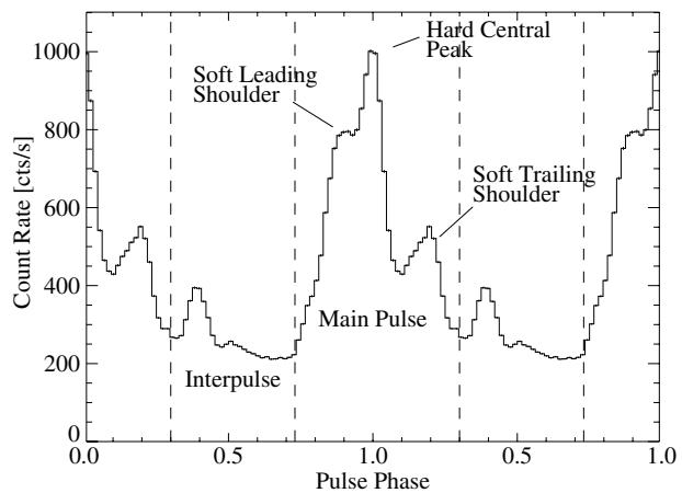
Fig. 4. Nomenclature for the different features of the Her X-1 pulse profile. This pulse profile is taken from orbit 30 in the energy range of 9.0–13.0 keV.
