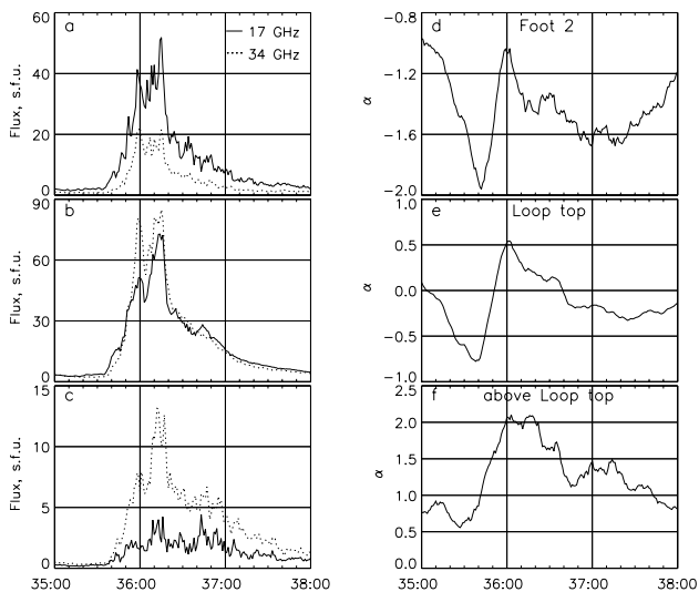
Fig. 8. Left panels: convolved and integrated radio fluxes coming from the 10'' \times 10'' boxes situated at the centre of the Northern HXR source (the loop footprint, panel a), at the centre of the 34 GHz source (panel b) and at the region 20'' eastward, i.e. over the loop (panel c). Right panels: the time profiles of the spectral indices \alpha , calculated as \alpha = \log(F_{34}/F_{17})/\log(34/17) , where F_{34} and F_{17} are the fluxes measured at the 34 GHz and 17 GHz bands, which characterise the spectral steepness, are shown in panels d, e and f (the regions correspond to the time profiles shown in panels a), b) and c)).
