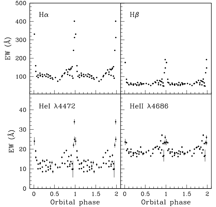
Fig. 9. Equivalent width curves of H \alpha , H \beta , He I \lambda 4472, and He II \lambda 4686 as a function of orbital phase. No phase binning has been applied and a full orbital cycle has been repeated for continuity.
