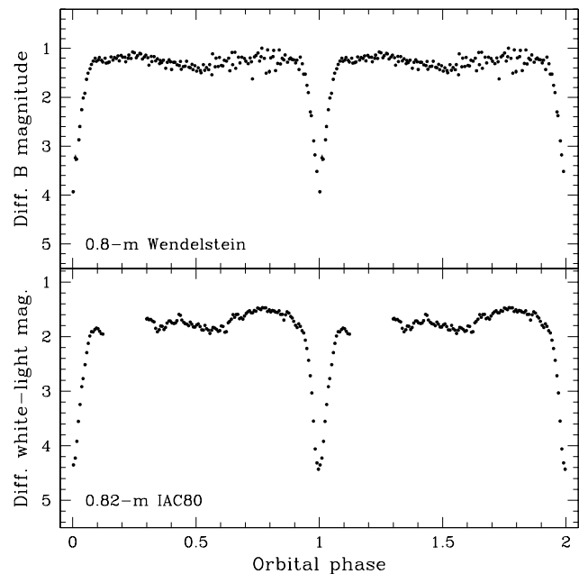
Fig. 3. Average light curves of HS 0728+6738. The individual data points were averaged into 150 phase bins. A full orbital cycle has been plotted twice.
