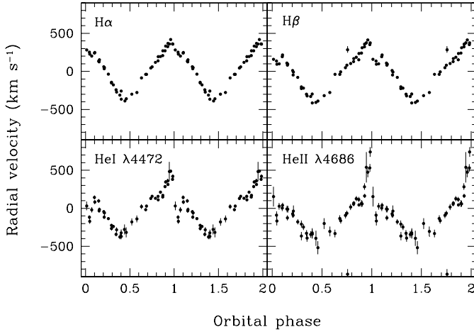
Fig. 8. Radial velocity curves of H \alpha , H \beta , He I \lambda 4472, and He II \lambda 4686 as a function of orbital phase. No phase binning has been applied and a full orbital cycle has been repeated for continuity.
