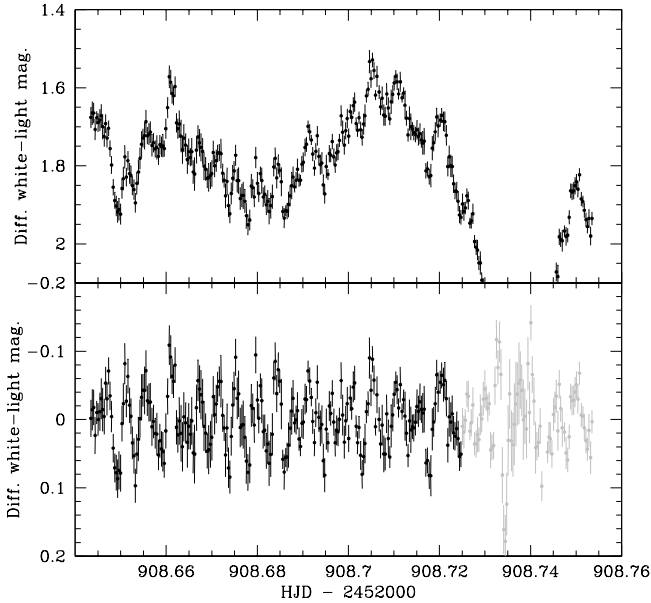
Fig. 4. Top panel: out-of-eclipse variability on the 2003 September 25 light curve (IAC80 telescope). A short-period oscillation with a time scale of 7–10 min is easily spotted. Bottom panel: same light curve detrended for period analysis. The points plotted in grey lie in the orbital phase interval 0.9–1.1. See text for details.
