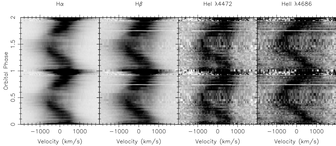
Fig. 10. Trailed spectra of H\alpha , H\beta , He\ I\ \lambda 4472 , and He\ II\ \lambda 4686 . No phase binning has been applied. Black represents emission and a full orbit has been repeated for clarity.
