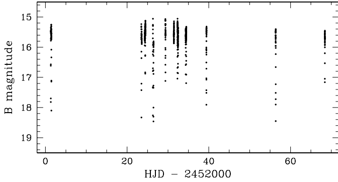
Fig. 6. Long-term B -band light curve of HS 0728+6738 from the Wendelstein observations. The measurements span approximately 67 days. An average value of B \sim 15.6 is observed outside of eclipse. The large change in eclipse depth is not real but due to missing data points at mid-eclipse in many of the light curves.
