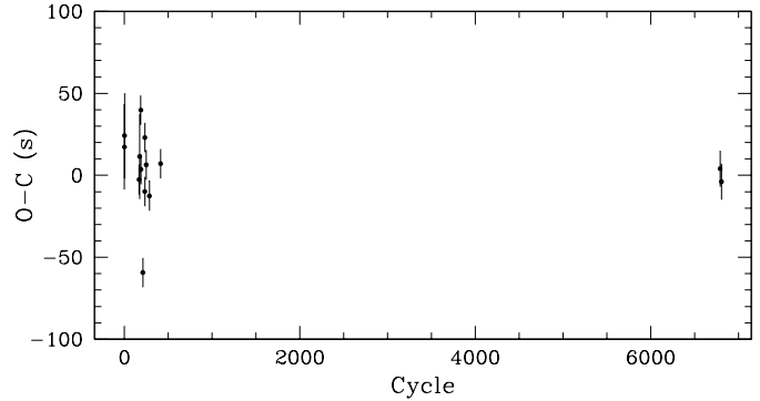
Fig. 2. O-C diagram of the eclipse timings. The errors have been determined by propagating the errors in the measurement of the mid-eclipse times and the corresponding error from the ephemeris.
