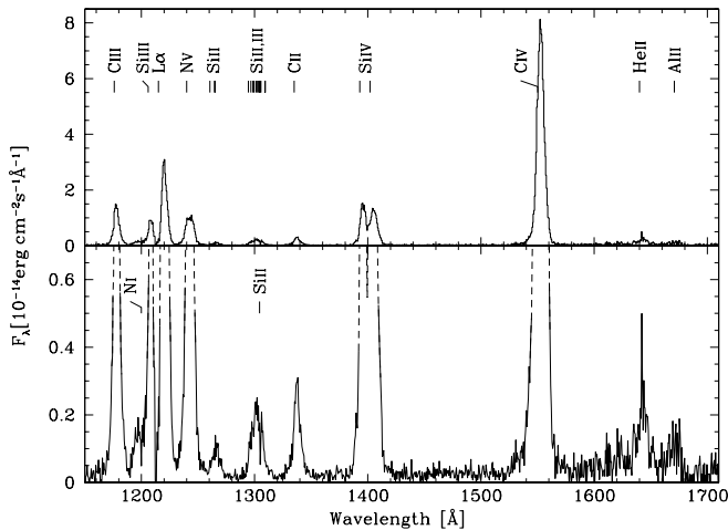
Fig. 11. HST/STIS far-ultraviolet spectrum of HS 0728+6738 taken at mid-eclipse. Note the absence of significant continuum flux and the strong emission lines.
