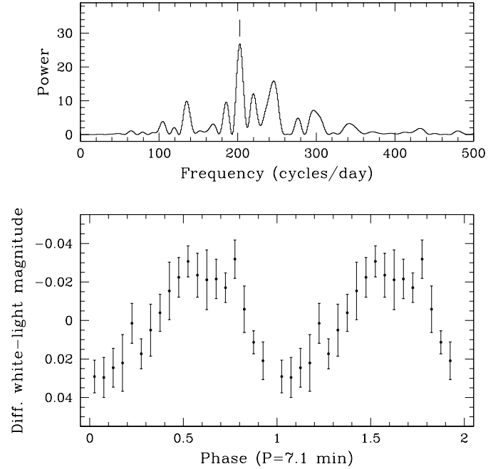
Fig. 5. Top panel: Scargle periodogram of the 2003 September 25 light curve (IAC80 telescope) after eliminating the eclipse and detrending. The strongest peak is centred at 7.1 min. Bottom panel: the light curve folded on the 7.1-min period after averaging the data into 20 phase bins (the average value has been subtracted). A complete cycle has been repeated for continuity.
