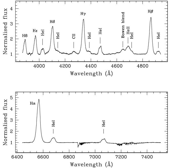
Fig. 7. Blue and red average spectra of HS 0728+6738.
