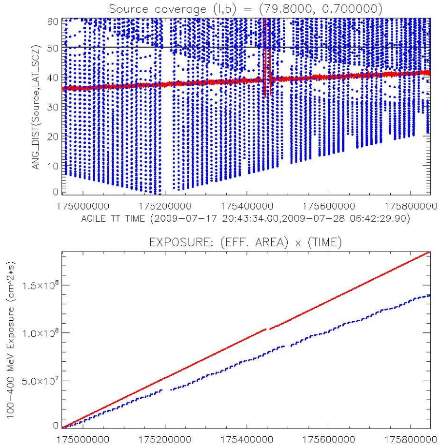
Fig. 7. Different pointing strategies of Cyg X-3 for AGILE-GRID (in red) and Fermi-LAT (in blue). Upper panel: time evolution of the instrument off-axis angle with respect to the fixed Cyg X-3 position during the period 2009 Jul 18-28 when the AGILE operates in pointing mode. The curve in blue show the off-axis angle evolution for the all-sky scanning pointing strategy of Fermi-LAT. The curve in red show the off-axis angle for the AGILE-GRID fixed pointing strategy in 2009 Jul. Bottom panel: time evolution of the cumulative exposure between 100 MeV and 400 MeV for Fermi-LAT (blue curve, using public data and Pass 6 Version 3 Front photons Instrument Response Function) and AGILE-GRID (red curve) assuming a starting time on 2009 Jul 18.
