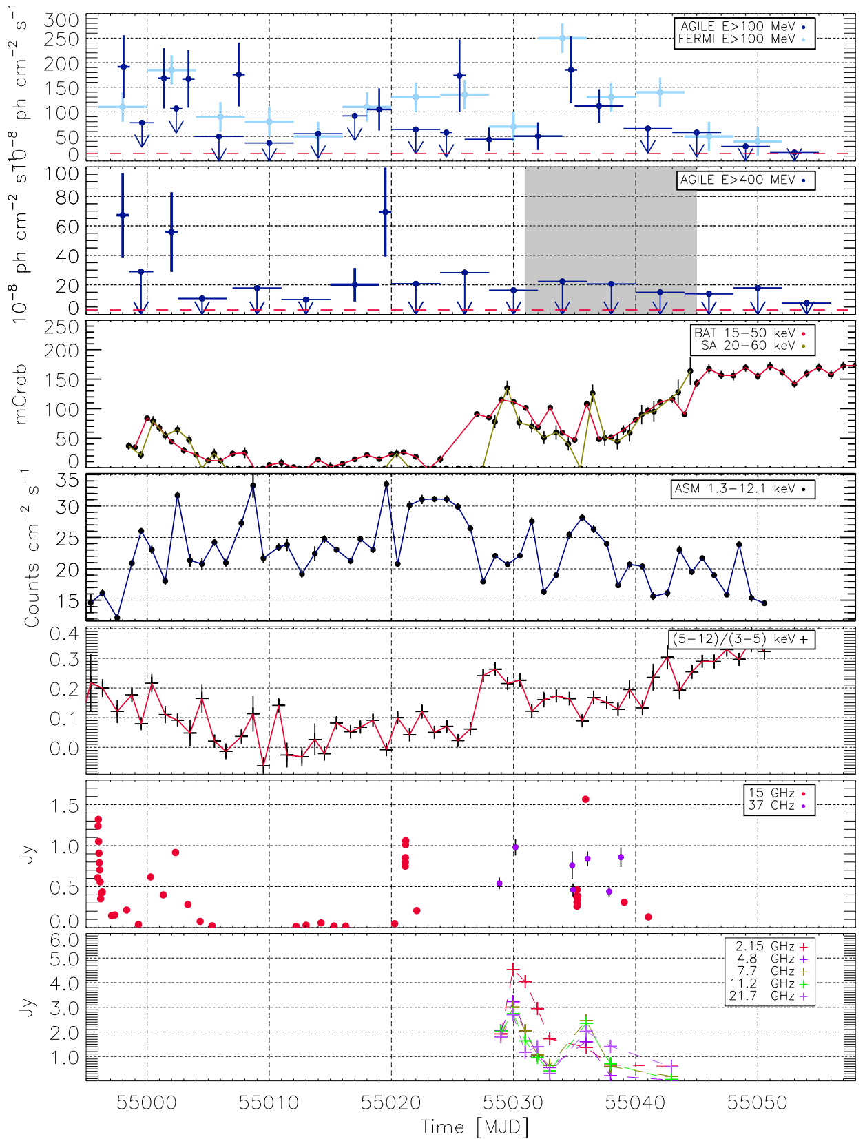
Fig. 3. AGILE/GRID, AGILE/SA, Fermi/LAT, Swift/BAT, XTE/ASM, AMI-LA, RATAN-600 and Metsähovi Radio Observatory data of Cyg X-3 during the uninterrupted 2-months period 2009 Jun.–Jul. (Panel 1 (top)) the AGILE-GRID \gamma -ray light curve with a variable window time to put in evidence the Cyg X-3 flares of 1-day timescale, the other data and upper-limits are determined with 1- 2- or 4-day time intervals; the Fermi light curve of 4-days timescale. E > 100 MeV. (Panel 2) the AGILE-GRID \gamma -ray light curve for E > 400 MeV and the coverage of MAGIC observation (gray area). (Panel 3) the hard X-ray light curve as monitored by BAT (15-50 keV) and by Super-AGILE (20-60 keV) with a daily timescale bin. (Panel 4) the soft X-ray light curve as monitored by XTE-ASM (1.3-12.1 keV) for a 1-day integration time bin; (Panel 5) the ASM hardness ratio (5 – 12keV)/(3 – 5keV) data. (Panel 6) AMI-LA radio flux monitoring of Cyg X-3 at 15 GHz and the Metsähovi Radio Observatory data at 37 GHz. (Panel 7) RATAN-600 radio telescope data at different frequencies. The AGILE/GRID \gamma -ray upper limits are at the 2 - \sigma level, the flux error bars are 1 - \sigma values.
