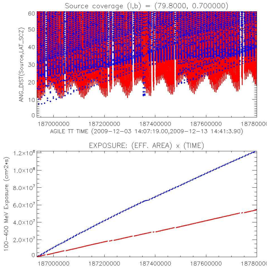
Fig. 8. Same pointing strategies of Cyg X-3 for AGILE-GRID (in red) and Fermi-LAT (in blue). Upper panel: time evolution of the instrument off-axis angle with respect to the fixed Cyg X-3 position during the period 2009 Dec. 3-13, when AGILE started to operate in spinning mode. The curves show the off-axis angle evolution for the all-sky scanning pointing strategy of AGILE GRID (in red) and Fermi-LAT (in blue). Bottom panel: time evolution of the cumulative exposure between 100 MeV and 400 MeV for Fermi-LAT (blue curve, using public data and Pass 6 Version 3 Front photons Instrument Response Function) and AGILE-GRID (red curve) assuming a starting time on 2009 Dec. 3.
