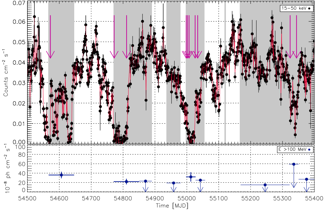
Fig. 1. (Top panel) Swift /BAT lightcurve (in counts per second in the energy range 15-50 keV) and AGILE-GRID \gamma -ray flares for E > 100 MeV as a function of time. The red arrows mark the dates of major \gamma -ray flares of Cyg X-3 : MJD 54572, 54772, 54811, 54998, 55001, 55003, 55007, 55025, 55034, 55324, 55343. Gray areas show the interval of good AGILE \gamma -ray exposure of Cyg X-3 . (Bottom panel) Average \gamma -ray flux from Cyg X-3 region in hard and soft X-ray state for E > 100 MeV.
