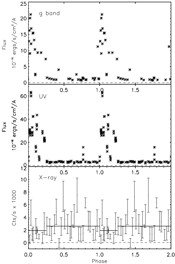
Figure 4. The light curves of KL Dra made at three wavebands folded on a period of 61.5 days with a T_0 = \text{MJD } 55173.4 .
