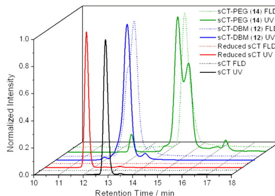
Figure 2. RP-HPLC analysis of the sCT-DBM conjugation reactions, with simultaneous UV ( \lambda = 280 \text{ nm} ) and fluorescence ( \lambda_{\text{ex}} = 341 \text{ nm} , \lambda_{\text{em}} = 502 \text{ nm} ) detection.
