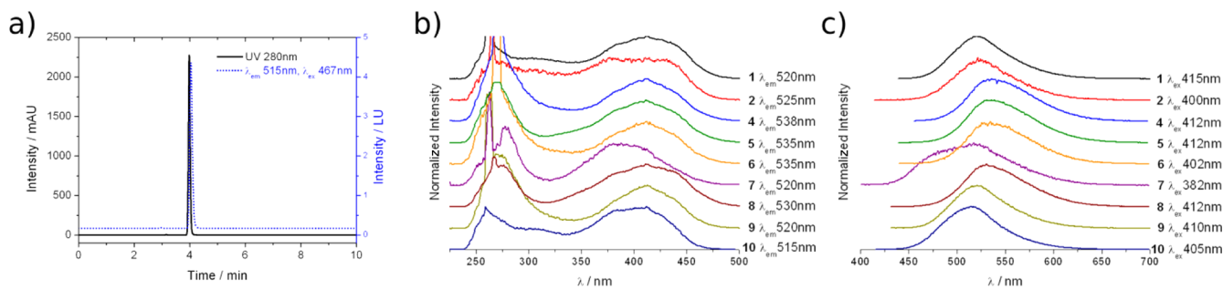
Figure 1. (a) HPLC chromatogram of 1 with simultaneous UV ( \lambda = 280 nm) and fluorescence ( \lambda_{ex} = 467 nm, \lambda_{em} = 515 nm) detection. (b) Excitation spectra and (c) emission spectra of fluorescent DTMs 1–10.
