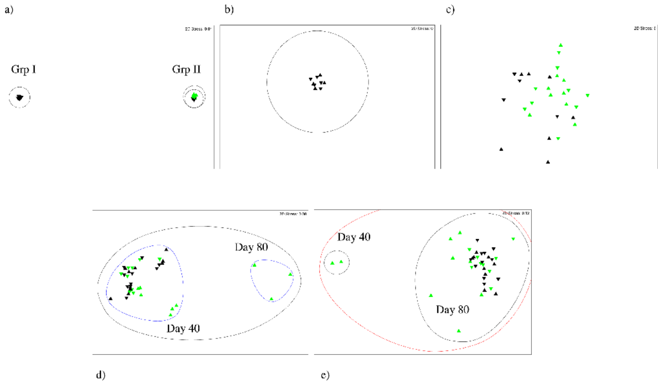
Figure 2. Development of phototroph, bacterial and fungal communities in Gartenacker soil. Phototroph (23S rRNA genes of plastids), bacterial (16S rRNA) and fungal (ITS) community structure at the surface (m) and bulk (!) of a pasture soil under light (green) and dark (black) conditions: (a) phototrophs all samples; (b) phototrophs close up of Grp I samples; (c) phototrophs close up of Grp II samples; (d) bacteria all samples (e) fungi all samples. Non-metric dimensional scaling shows clustering based on the similarity of microbial community structure between treatments: 15% (red cluster), 40% (black cluster) and 85% (blue cluster). doi:10.1371/journal.pone.0069048.g002
