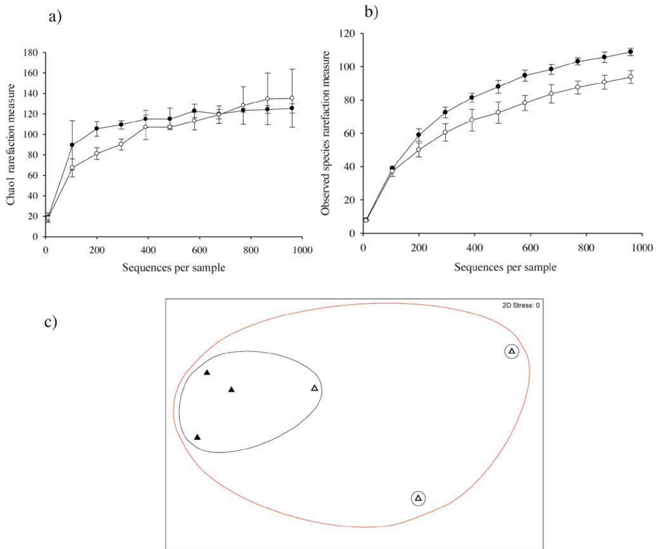
Figure 7. Fungal diversity at the soil surface under light and dark conditions. a diversity estimates Chao1 (a) and Observed Species (b) and non-metric multidimensional scaling of community structure similarity (c) for fungi (ITS region) at the soil surface of a pasture soil after 80 days incubation under light (open symbols) or dark (closed symbols) conditions. OTU clustering was performed at the 97% similarity threshold using UCLUST. Error bars are \pm 1 S.E. Non-metric multidimensional scaling shows clustering based on the similarity of microbial community structure between treatments: 55% (red cluster) and 70% (black cluster). doi:10.1371/journal.pone.0069048.g007
