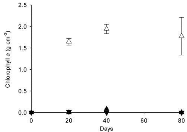
Figure 1. Chlorophyll a development in Gartenacker soil. Chlorophyll a in the surface (m) and bulk (.) of pasture soil after incubation under light (open symbols) or dark (closed symbols) conditions. Errors bars are \pm 1 standard error. doi:10.1371/journal.pone.0069048.g001
