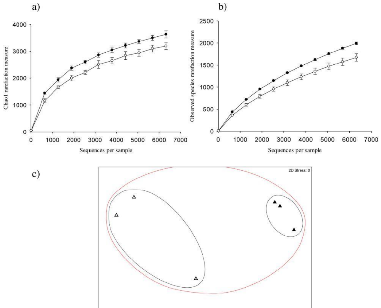
Figure 5. Bacterial diversity at the soil surface under light and dark conditions. a diversity estimates Chao1 (a) and Observed Species (b) and non-metric multidimensional scaling of community structure similarity (c) for bacteria (16S rRNA) at the soil surface of a pasture soil after 80 days incubation under light (open symbols) or dark (closed symbols) conditions. OTU clustering was performed at the 97% similarity threshold using uclust. Error bars are \pm 1 S.E. Non-metric multidimensional scaling shows clustering based on the similarity of microbial community structure between treatments: 45% (red cluster) and 55% (black cluster). doi:10.1371/journal.pone.0069048.g005
