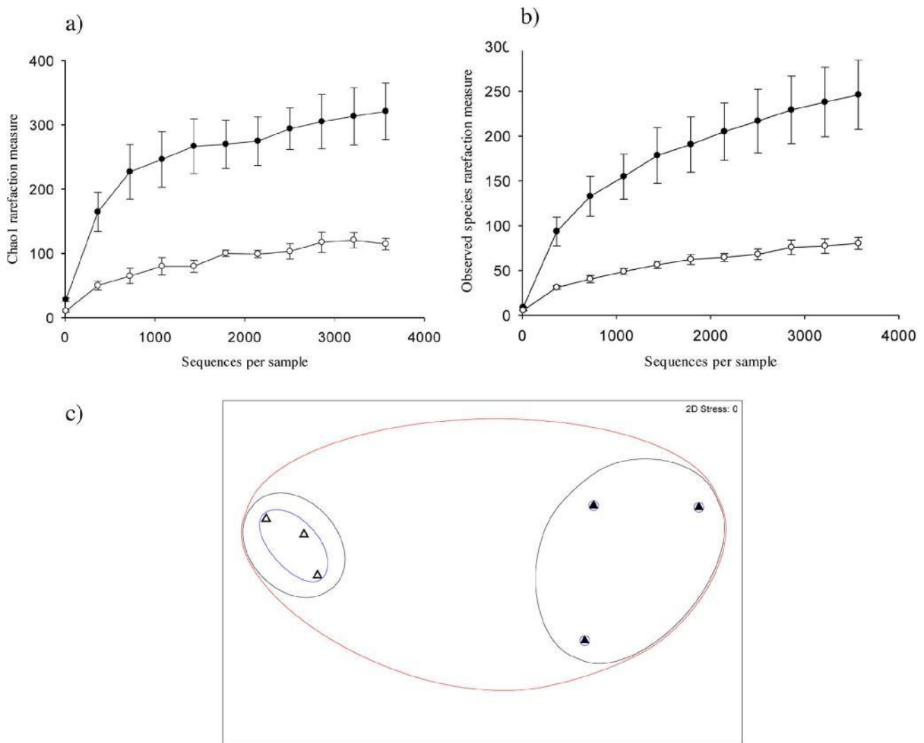
Figure 3. Phototroph diversity at the soil surface under light and dark conditions. a diversity estimates Chao1 (a) and Observed Species (b) and non-metric multidimensional scaling of community structure similarity (c) for phototrophs (23S rRNA genes of plastids) at the soil surface of a pasture soil after 80 days incubation under light (open symbols) or dark (closed symbols) conditions. OTU clustering was performed at the 97% similarity threshold using UCLUST. Error bars are \pm 1 S.E. Non-metric multidimensional scaling shows clustering based on the similarity of microbial community structure between treatments: 20% (red cluster), 25% (black cluster) and 80% (blue cluster). doi:10.1371/journal.pone.0069048.g003
