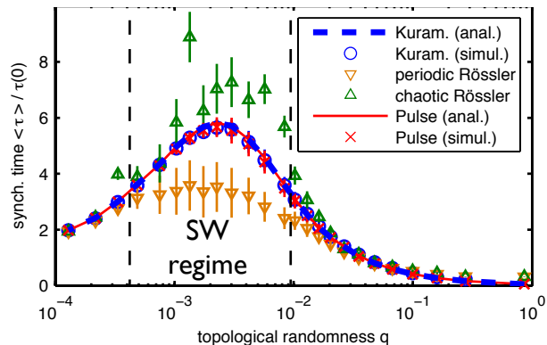
Fig. 4: (color online) Synchronization is slowest in the small world regime for various oscillator types and coupling schemes (network parameters as in Fig. 2). Normalized average synchronization times \langle \tau \rangle / \tau(0) vs. q for Kuramoto, pulse-coupled and periodic as well as chaotic Rössler oscillators (network topologies as in Fig. 2). Neurons with delayed pulse-coupling: I = 1.01 , \gamma = 1 , J = -0.2 , \tau = 0.1 ; Diffusively coupled Rössler oscillators: a = 0.2 , c = 5.7 , periodic: b = 1.7 , J = 2 , chaotic: b = 0.2 , J = 6 . The synchronization times are determined by measuring the distances d = \max_{i,j} \{((x_i - x_j)^2 + (y_i - y_j)^2 + (z_i - z_j)^2)^{1/2}\} (Rössler), and d = \max_i |\delta_i| (pulse-coupled) and fitting (4).
