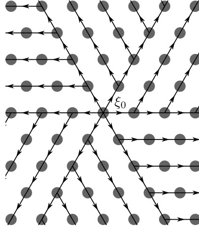
FIGURE 6. An illustration of the definition of \Gamma_\xi .
