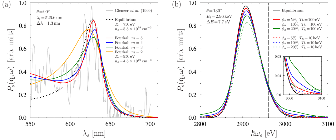
Figure 1. (a) Theoretical fit to plasmon data (noisy grey curve) in laser-produced Au plasma using the distribution of Fourkal et al. [10] for m = 5 (red curve), m = 4 (blue curve), m = 3 (green curve) and m = 2 , i.e. Maxwellian, (orange). The best fit constrained by equilibrium (black curve) is shown for comparison. (b) Theoretical power spectra for warm dense Be at T_e = 12\text{eV} and n_e = 3 \times 10^{23}\text{cm}^{-3} including a hot tail with T_h = 100\text{ eV} (solid curves) and T_h = 10\text{ keV} (dashed curves), and various weights \phi_h ; 5% (red curve), 10% (blue curve) and 20% (green curve) compared to an equilibrium calculation (black curve) [12].
