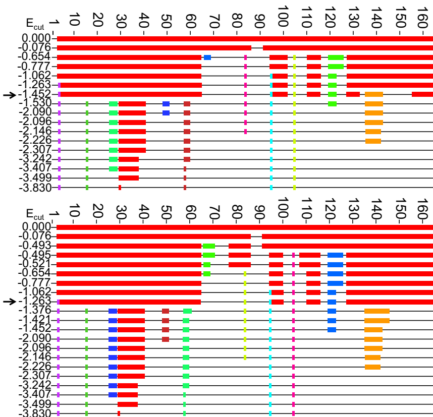
FIGURE 2 RD plots of the CypA-CsA complex ( upper ) and unbound CypA ( lower ). The RCD is shown at different values of E_{\text{cut}} (kcal/mol). Rigid residues are shown as thick colored blocks and flexible regions as thin horizontal black lines. Residues that are mutually rigid are shown in the same color. The line representing the FIRST folding core in each case is indicated by an arrow. To see this figure in color, go online.
