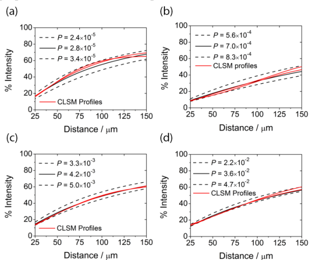
Figure 6. Experimental and corresponding simulated fluorescence-distance plot for (a) 100 mM acetic acid, (b) 100 mM propanoic acid, (c) 10 mM butanoic acid and (d) 10 mM hexanoic acid. The permeation coefficients corresponding to the upper and lower bounds and best fit of the CLSM data are shown (units \text{cm s}^{-1} ).
