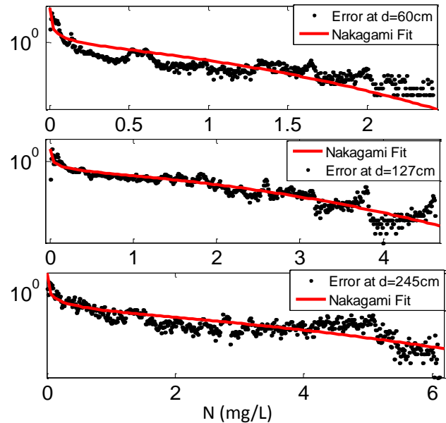
Fig. 1. Noise (error) PDF with fitted Nakagami distributions (Log Scale)
