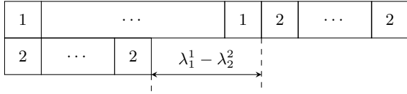
Figure 2.2: The quantity \lambda_1^1 - \lambda_2^2 in the exponent in Example 2
