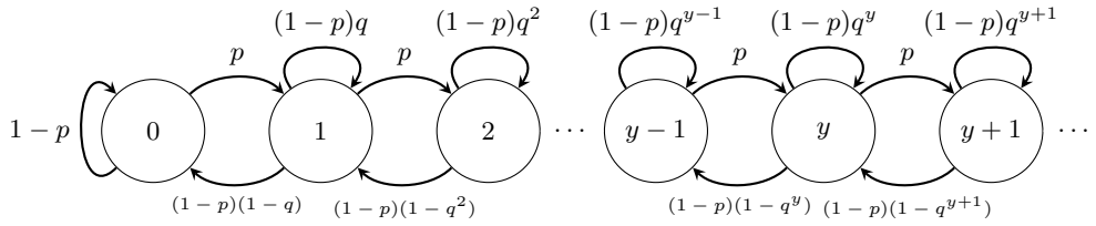
Figure 2.5: The birth-and-death process Y
