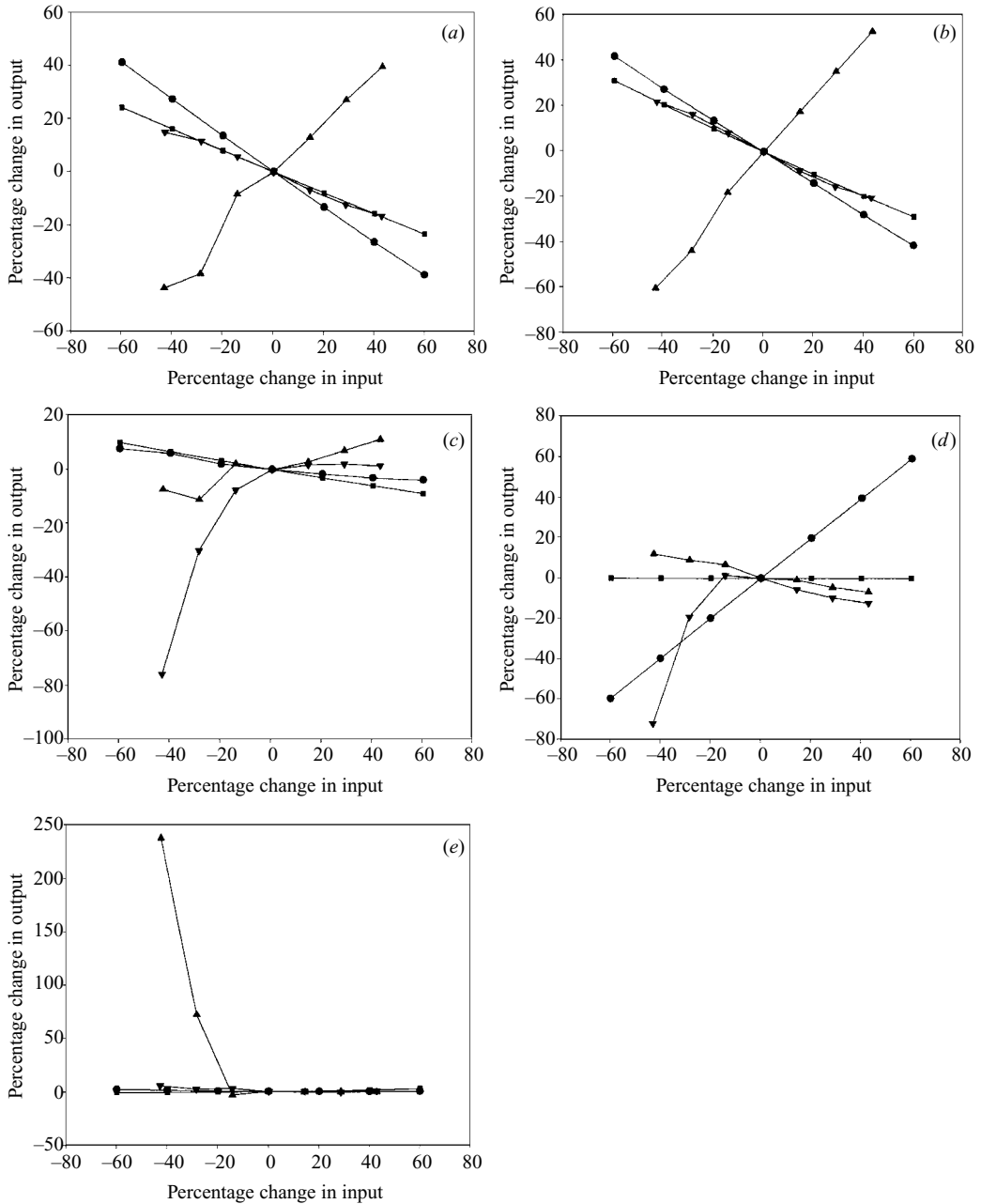
Fig. 2. Effects of variation in individual input factors on (a) applied nitrogen to achieve 99% of maximum dry weight, for average rainfall on sandy loam soil, (b) increase in dry weight at optimum applied N relative to that at zero applied N, for average rainfall on sandy loam soil, (c) the amount of \text{NO}_3\text{-N} leached from 0-30 cm, for high rainfall on sandy soil, (d) the amount of \text{NO}_3\text{-N} leached from 0-90 cm, for high rainfall on sandy soil, and (e) soil mineral N in 0-30 cm at harvest, for average rainfall on sandy loam soil. Effects shown for soil mineral N (●), mineralization rate (■), yield expectation (▲) and crop duration (▼). Mid-point values are given in Appendix A.
