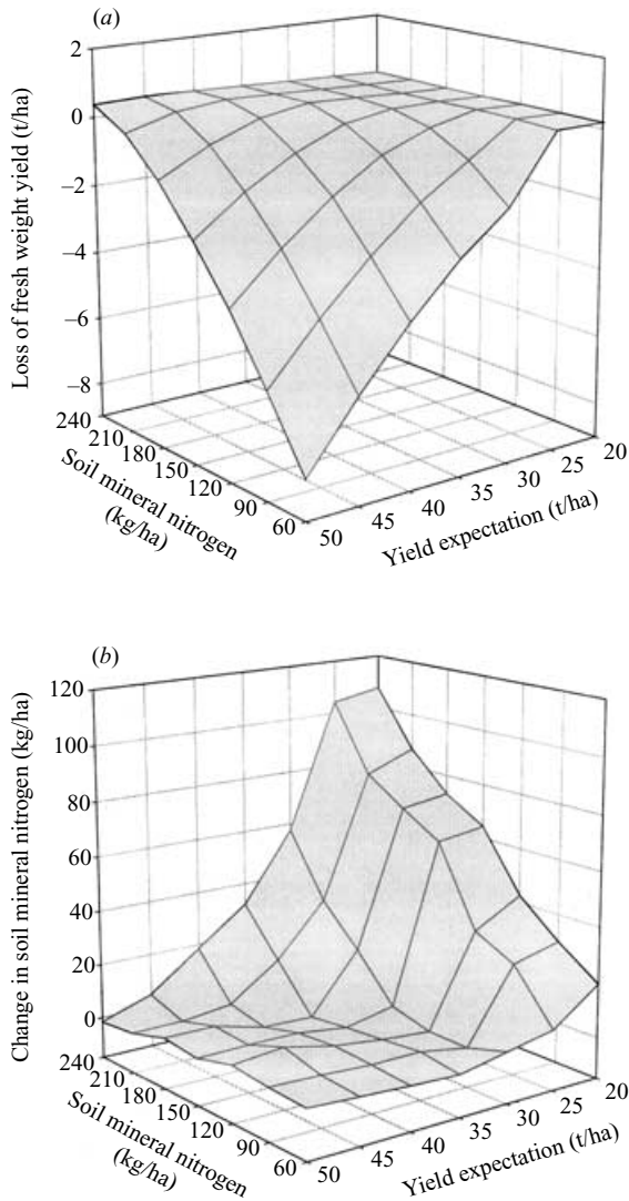
Fig. 4. The impact of incorrect values of soil mineral N and yield expectation on (a) achieved fresh weight yield and (b) soil mineral N at harvest in 0–90 cm. Applied N (147 kg/ha N) based on 150 kg/ha mineral N, a yield expectation of 35 t/ha for average rainfall, a crop duration of 98 days, and a mineralization rate of 0.70 kg/ha/day @ 15.9 °C on sandy loam soil.
