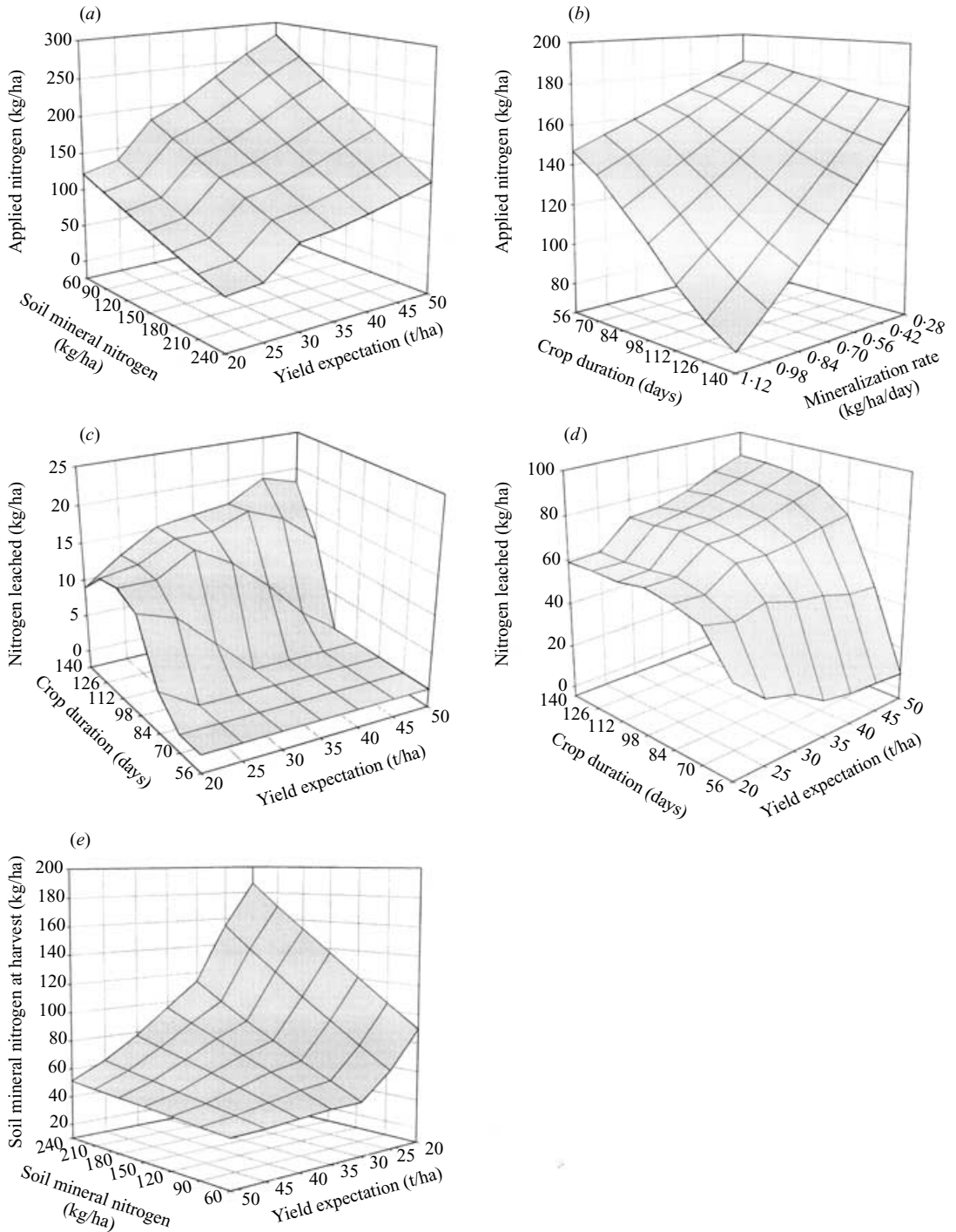
Fig. 3. Effects of joint variation of (a) soil mineral N and yield expectation on applied N to achieve 99% of maximum dry weight, for average rainfall on sandy loam soil, (b) mineralization rate and crop duration on applied N to achieve 99% of maximum dry weight, for average rainfall on sandy loam soil, (c) yield expectation and crop duration on the amount of \text{NO}_3\text{-N} leached from 0–30 cm, for average rainfall on sandy soil, (d) yield expectation and crop duration on \text{NO}_3\text{-N} leached from 0–30 cm, for high rainfall on sandy soil, and (e) soil mineral N and yield expectation on soil mineral N in 0–90 cm at harvest, for average rainfall on sandy loam soil.
