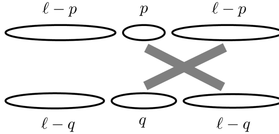
Fig. 1. The p\ell + q\ell - 2pq edges of K_{[\ell,p,q]} corresponding to factors bounded from above by d + \varepsilon_2 in (19).
