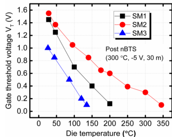
Fig. 5. Post nBTS temperature dependence of threshold voltage V_T following the 30 minute -5 V nBTS test period at 300 °C. These results illustrate the situation that could occur if V_T drifts too far in a negative direction; the devices may enter a normally-on state.
