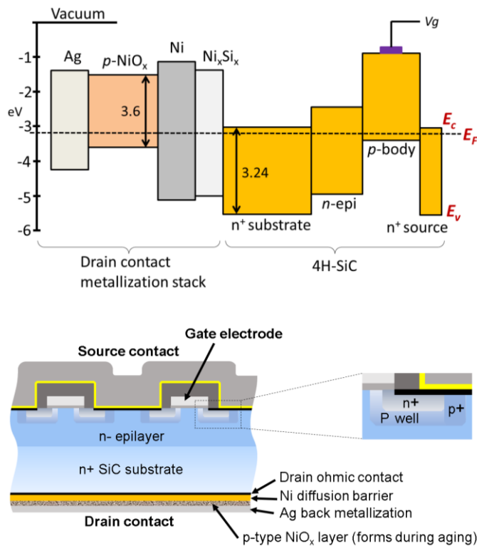
Fig. 13. Band energy alignment diagram and associated simplified SiC D-MOSFET device structure, indicating the position of the \text{NiO}_x layer that appeared on the back of the drain contact metallization stack.
