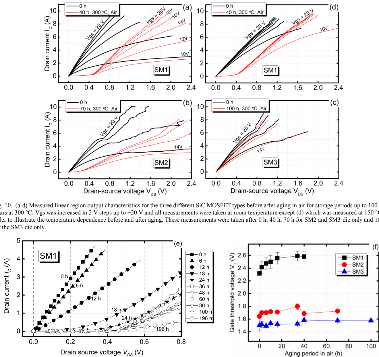
Fig. 10 (e) Aging time period dependence of the output characteristics for up to 196 hours to illustrate the change versus aging time a long time after the rectifying output becomes evident. (f) Threshold voltage shifts due to aging in air at 300 °C for up to 100 hours. In this case, single-shot measurements were taken carefully to limit the possibility of further measurement pulses influencing the results.
