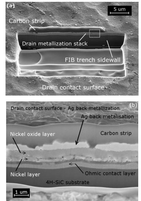
Fig. 12. (a) Tilted surface SEM image of one of a number of FIB trenches milled in the drain side of the SM2 die after heating for 1000 hours in N_2 . (b) Cross section SEM image of drain contact metallization stack taken from the FIB trench sidewall, indicating the formation of a nickel oxide layer under the silver.
