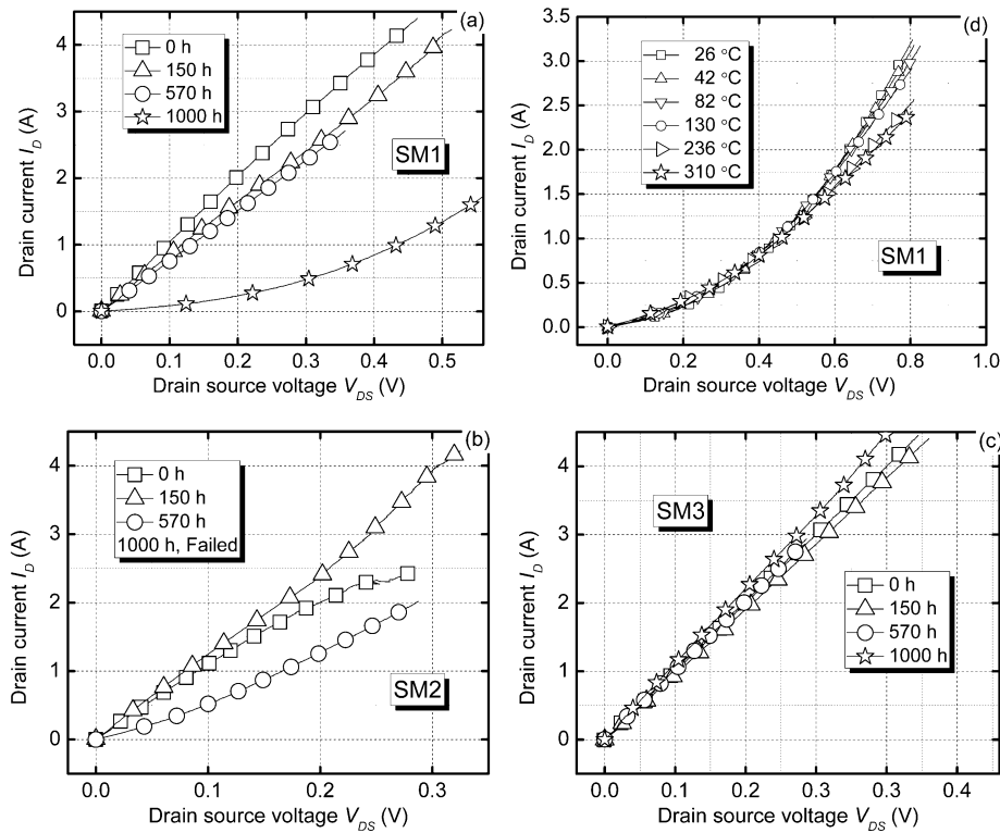
Fig. 11. (a-c) Measured linear region output characteristics versus inert N_2 atmosphere storage period at 300 °C for the three different SiC MOSFET device types. All measurements were taken at room temperature and for a gate voltage of +20 V. (d) Temperature dependence of output characteristics for the SM1 die after storage in N_2 atmosphere for 1000 hours at 300 °C.
