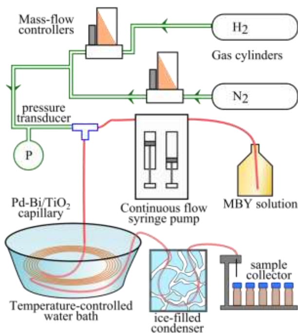
Fig. 3. Scheme of the hydrogenation apparatus
