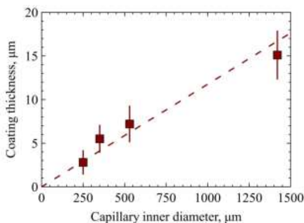
Fig. 7. Effect of the capillary inner diameter on the coating thickness (SEM data) using a 80 g/L TiO 2 sol.
