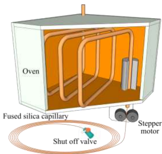
Fig. 2. Schematic view of the coating apparatus.
