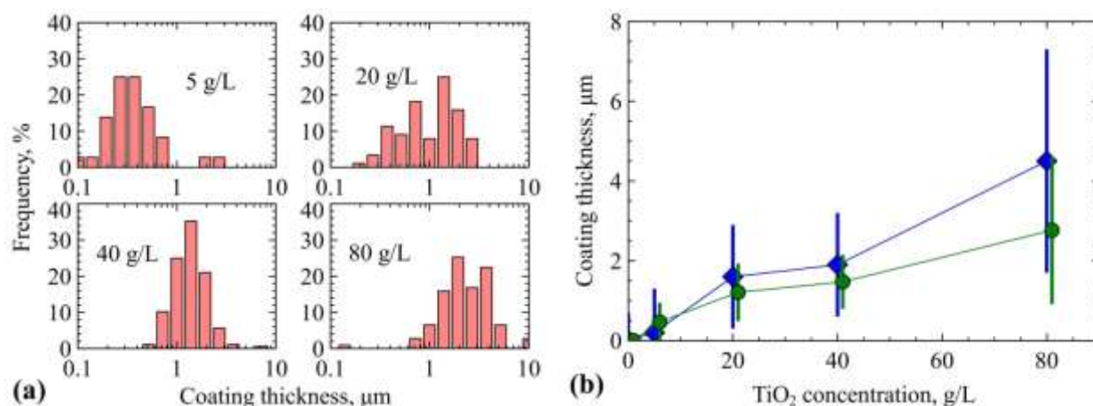
Fig. 6. (a) Distribution of the TiO 2 coating thickness obtained in the 250 μm fused silica capillaries using different precursor sol concentrations. Displacement speed: 0.2 mm/s. Oven temperature: 450 K. (b) The comparison of the average coating thickness determined by (●) SEM and (◆) hydrodynamic study.
