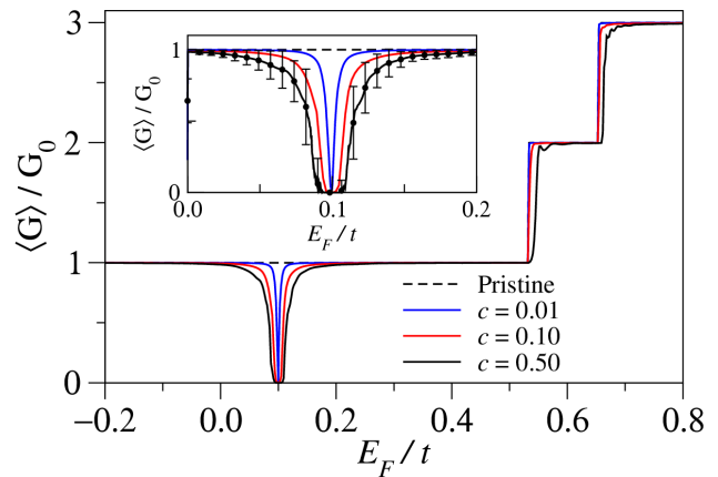
FIG. 2. (Color online) Average conductance as a function of the Fermi energy of a silicene nanoribbon when M = 0 . Solid lines correspond to the average over 100 realizations of random samples with adatom concentration c = 0 (pristine), 0.01, 0.10 and 0.50. The energy level of the adatom is \varepsilon_{\text{ad}} = 0.10t and the hopping parameter t_{\text{ad}} = 0.10t with t = 1.6 eV. The inset shows an enlarged view of the anti-resonance. Only the error bars of the more disordered sample ( c = 0.5 ) are displayed for clarity. Fluctuations strongly diminish upon lowering c .
