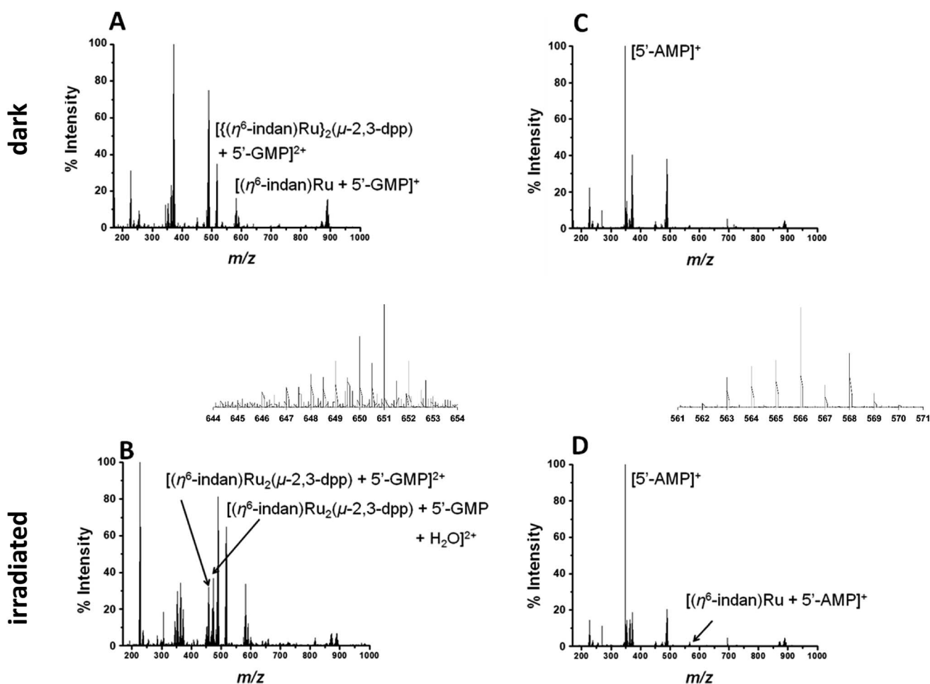
Fig. 3 (A and B) PCF-MS of 250\text{ }\mu\text{M} 1 and 500\text{ }\mu\text{M} 5' -GMP in DDW. Spectrum (A) dark solution peak at 517.6\text{ m/z} assigned as [(\eta^6\text{-indan})\text{Ru}_2(\mu\text{-}2,3\text{-dpp}) + 5'\text{-GMP}]^{2+} , the species at 582.03\text{ m/z} is [(\eta^6\text{-indan})\text{Ru} + 5'\text{-GMP}]^+ , and spectrum (B) is after 12\text{ s} of irradiation at 488\text{ nm} in the HC-PCF flow reactor, new peaks 640.04\text{ m/z} and 649.04\text{ m/z} (shown in inset) are assigned as [(\eta^6\text{-indan})\text{Ru}_2(\mu\text{-}2,3\text{-dpp}) + 2(5'\text{-GMP})]^{2+} and [(\eta^6\text{-indan})\text{Ru}_2(\mu\text{-}2,3\text{-dpp}) + 2(5'\text{-GMP}) + \text{H}_2\text{O}]^{2+} , respectively. (C and D) PCF-MS of 250\text{ }\mu\text{M} 1 and 500\text{ }\mu\text{M} 5' -AMP in DDW. Spectrum (C) dark solution, a peak is detected at 348.07\text{ m/z} ( [5'\text{-AMP} + \text{H}]^+ ), and spectrum (D) is after 12\text{ s} of irradiation at 488\text{ nm} in the HC-PCF flow reactor, the new peak at 566.04\text{ m/z} (shown in inset) is assigned as [(\eta^6\text{-indan})\text{Ru} + (5'\text{-AMP})]^+ .
