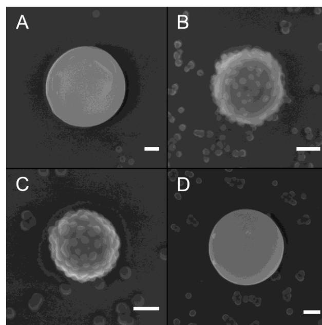
Figure 4. SEM images of the latex particles resulting from the Pickering emulsion polymerization of styrene a) in the absence of comonomer, in the presence of b) 1.0 wt% (with respect to styrene) and c) 3.0 wt% of di(ethylene glycol) ethyl ether acrylate, in the presence of d) 1.0 wt% of MAA. Additional pictures can be found in the supporting material ( Figure S4 ). Scale bars 100 nm.
