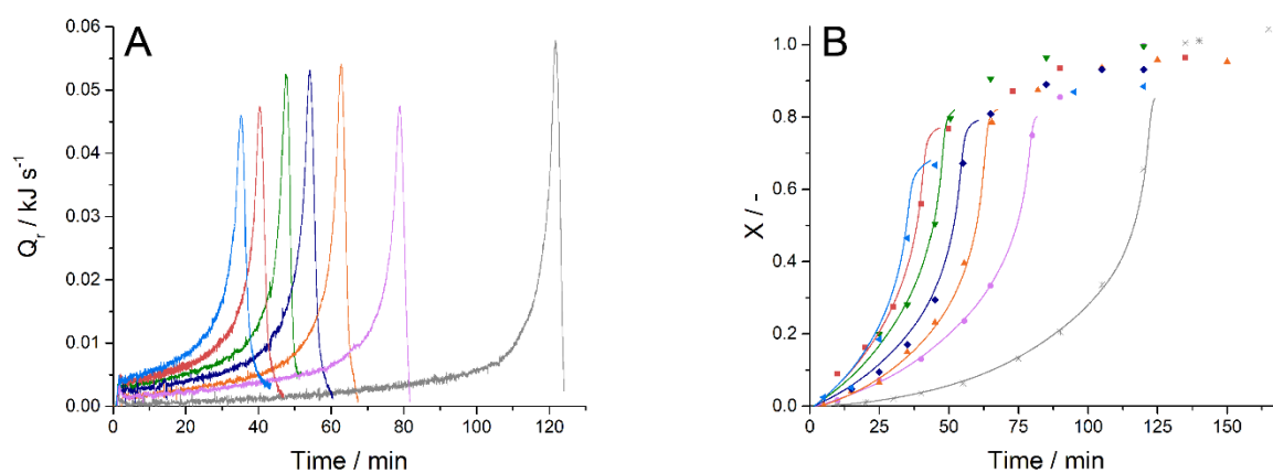
Figure 6. a) Variation of the heat of reaction ( Q_r ) for the Pickering emulsion polymerization of methyl methacrylate (MMA) in the presence of different initial nanosilica/MMA weight ratios ( \text{SiO}_2/\text{M} ); b) Estimated monomer conversion from calorimetry data (lines) compared to conversion measured from gravimetry samples withdrawn during the reaction (points). \text{SiO}_2/\text{M} = 0.00 (grey), 0.10 (pink), 0.50 (orange), 0.75 (dark blue), 1.00 (green), 1.50 (red), 2.00 (light blue) w/w.
