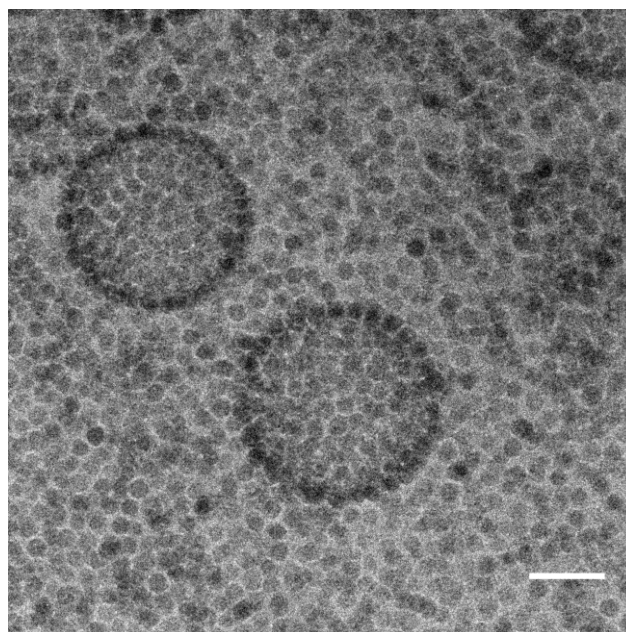
Figure 3. a) Cryo-TEM image of silica armoured MMA droplets in water obtained through sonication of a mixture of MMA and water in the presence of a silica nanosol (Ludox TM-40). Scale bar 100 nm.
