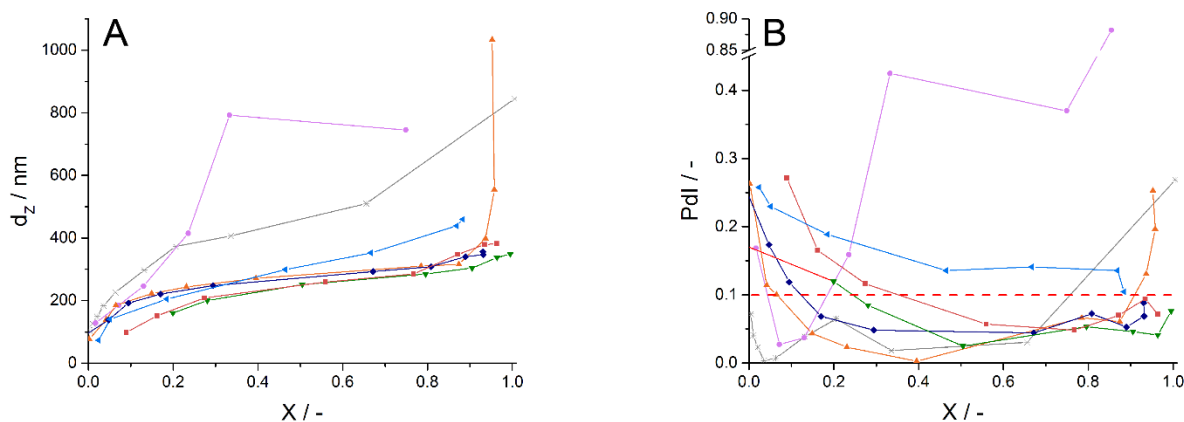
Figure 8. Pickering emulsion polymerization of MMA in the presence of different silica/monomer ratios ( \text{SiO}_2/\text{M} ); a) variation of the hydrodynamic diameter ( d_z ) with X ; b) variation of the particle dispersity ( Pdl ) with X . \text{SiO}_2/\text{M} = 0.00 (grey), 0.10 (pink), 0.50 (orange), 0.75 (dark blue), 1.00 (green), 1.50 (red), 2.00 (light blue) w/w.
