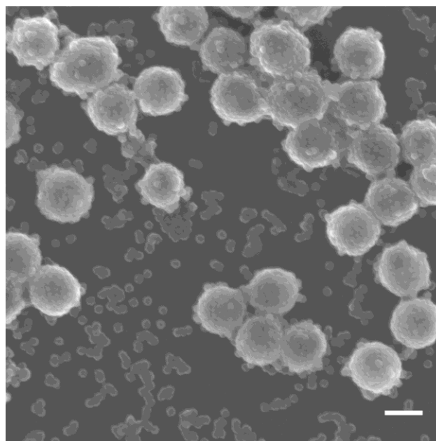
Figure 1. SEM image of PMMA-SiO 2 nanocomposite armoured latex particles obtained via Pickering emulsion polymerization. Scale bar 200 nm.
