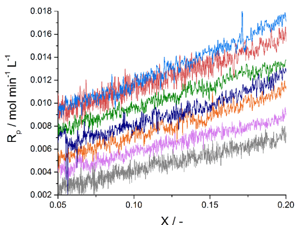
Figure 7. Variation in the polymerization rate ( R_p ) until 20% conversion for the Pickering emulsion polymerization of MMA in the presence of nanosilica. \text{SiO}_2/\text{M} = 0.00 (grey), 0.10 (pink), 0.50 (orange), 0.75 (dark blue), 1.00 (green), 1.50 (red), 2.00 (light blue) w/w. A broader look at the reaction rates until about 80% conversion can be found in the supporting material (Figure S6).
