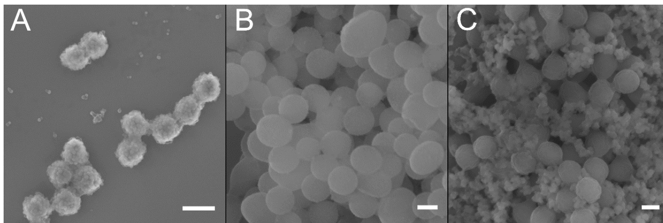
Figure 5. SEM pictures of latex nanoparticles formed in the case of a) \text{SiO}_2/\text{M}=1.50 w/w, b) \text{SiO}_2/\text{M} = 0.10 w/w, c) \text{SiO}_2/\text{M} = 0.00 w/w. Scale bars 300 nm.
