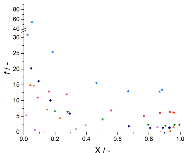
Figure 10. Variation of the ratio f (silica/nanocomposite particles surface area) as a function of monomer conversion ( X ) for the Pickering emulsion polymerization of MMA and nanosilica.
