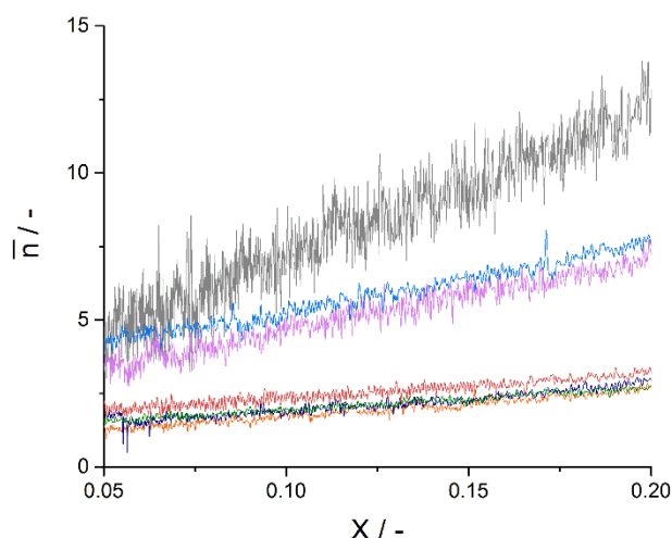
Figure 9. Variation in the average number of radicals per particle ( \bar{n} ) between 5 and 20% conversion for the Pickering emulsion polymerization of MMA in the presence of nanosilica. \text{SiO}_2/\text{M} = 0.00 (grey), 0.10 (pink), 0.50 (orange), 0.75 (dark blue), 1.00 (green), 1.50 (red), 2.00 (light blue) w/w.
