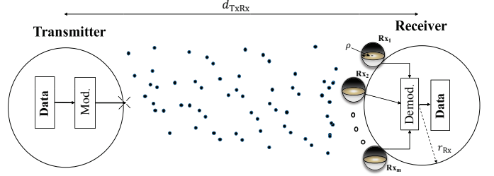
Fig. 1. System model. The fixed transmitter and receiver are located in the environment. The transmitter releases information molecules. These molecules diffuse based on Brownian motion. The receiver with multiple antennas can observe the number of molecules.
