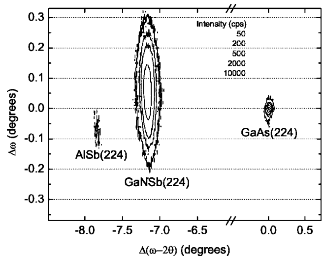
FIG. 2. Reciprocal space map of the 224 diffraction maxima from a 2- \mu m GaNSb epilayer grown on a 1- \mu m AlSb buffer layer on a GaAs substrate. This sample was grown at a temperature of 400 °C using a nitrogen plasma power of 200 W. Analysis of the 004 and 224 maps indicates that the anion sublattice of the GaNSb layer contains 0.78% N and that the epilayer is fully relaxed. The stated intensity values correspond to the contour lines in the map.
