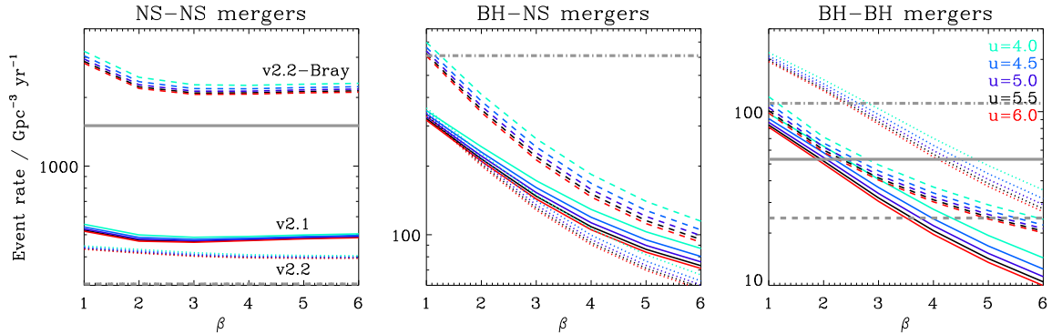
Figure 2. BPASS predictions for the merger rates of NS-NS, BH-NS and BH-BH mergers with different models with our different models. The solid lines are for model (i) v2.1, the dotted-lines are for model (ii) v2.2 and the dashed-lines for model (iii) v2.2 with the Bray kick. The solid horizontal grey lines indicate the best estimate for the merger rates from Abbott et al. (2016b, 2019a) while the dashed lines are the lower limits and the dash-dotted lines are the upper limits. For NS-NS, BH-NS and BH-BH mergers rates these are taken to be 1540^{+3200}_{-1200} , <610 and 53.2^{+58.5}_{-28.8} \text{Gpc}^{-3} \text{yr}^{-1} respectively.
