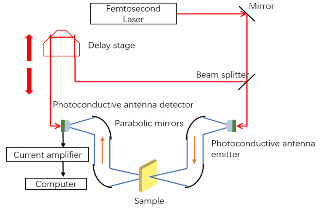
Fig.1. Diagram of the THz spectroscopy measurement in transmission geometry. The red line shows the route of the laser, the red orange arrows the route of the THz beam.
