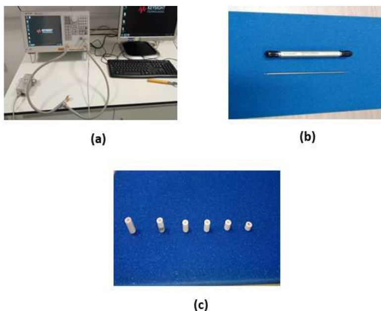
Figure S1. Dielectric measurement set up (a) VNA, (b) co-axial probe and (c) prepared VNA test samples
