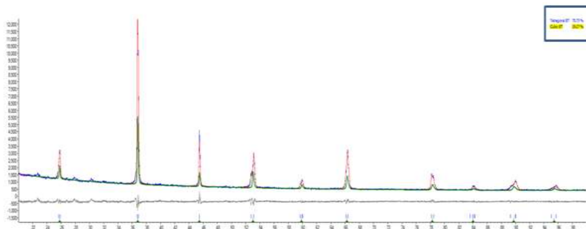
Figure S2. Rietveld analysis results for BaTiO 3 .
