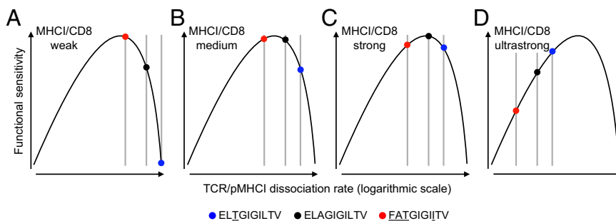
Fig. 3. Theoretical interpretation of the differential focusing effect mediated by CD8. Graphical representation of the differential focusing effect based on two key assumptions: 1) functional sensitivity depends nonmonotonically on the TCR/pMHC dissociation rate; and 2) the pMHC/CD8 interaction affects the TCR/pMHC dissociation rate by an invariant factor, equivalent to translation on a logarithmic scale ( SI Appendix ). (A–C) Modulation of the pMHC/CD8 interaction moves peptide ligands along this curve, altering the agonist hierarchy as a function of the TCR/pMHC dissociation rate. (D) A hypothetical ultrastrong pMHC/CD8 interaction would be expected to reverse the agonist hierarchy from FAT > ELA > 3T to FAT < ELA < 3T.
