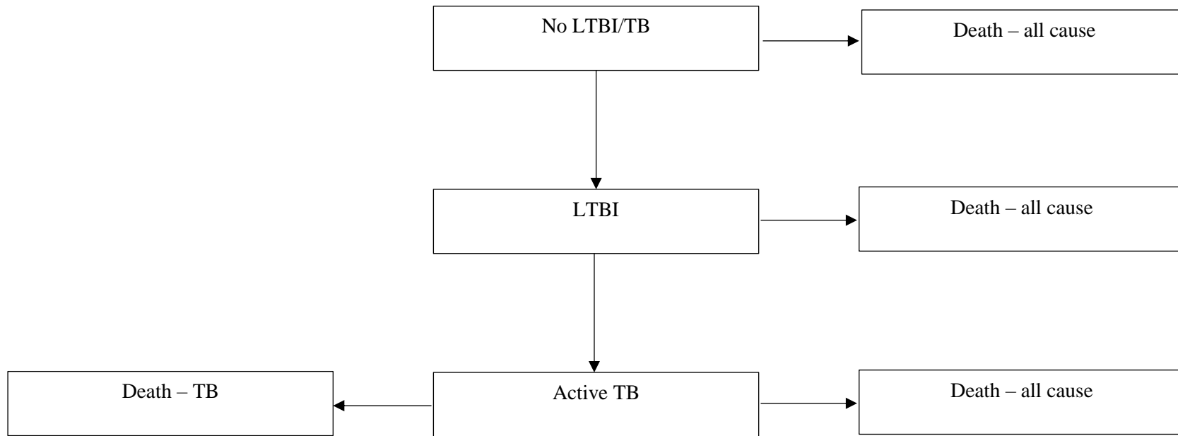
Appendix Figure 2: Markov model
