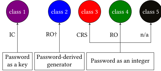
Figure 2: Taxonomy. IC: ideal cipher model. RO†: random oracle model assuming secure hash-to-group function (hash-to-curve in EC setting). CRS: common reference string model assuming a trusted setup. RO: random oracle model assuming secure one-way hash function. Finally, n/a denotes absence of a generally applicable model or established proofs (cf. Table 1).
