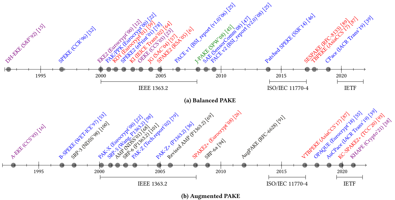
Figure 1: Timeline: PAKE protocols. Color-coding is based on the taxonomy explained in Section 3.
