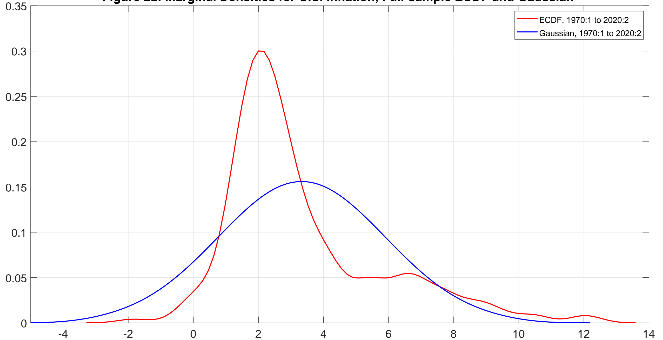
Figure 2a: Marginal Densities for U.S. Inflation, Full-sample ECDF and Gaussian
