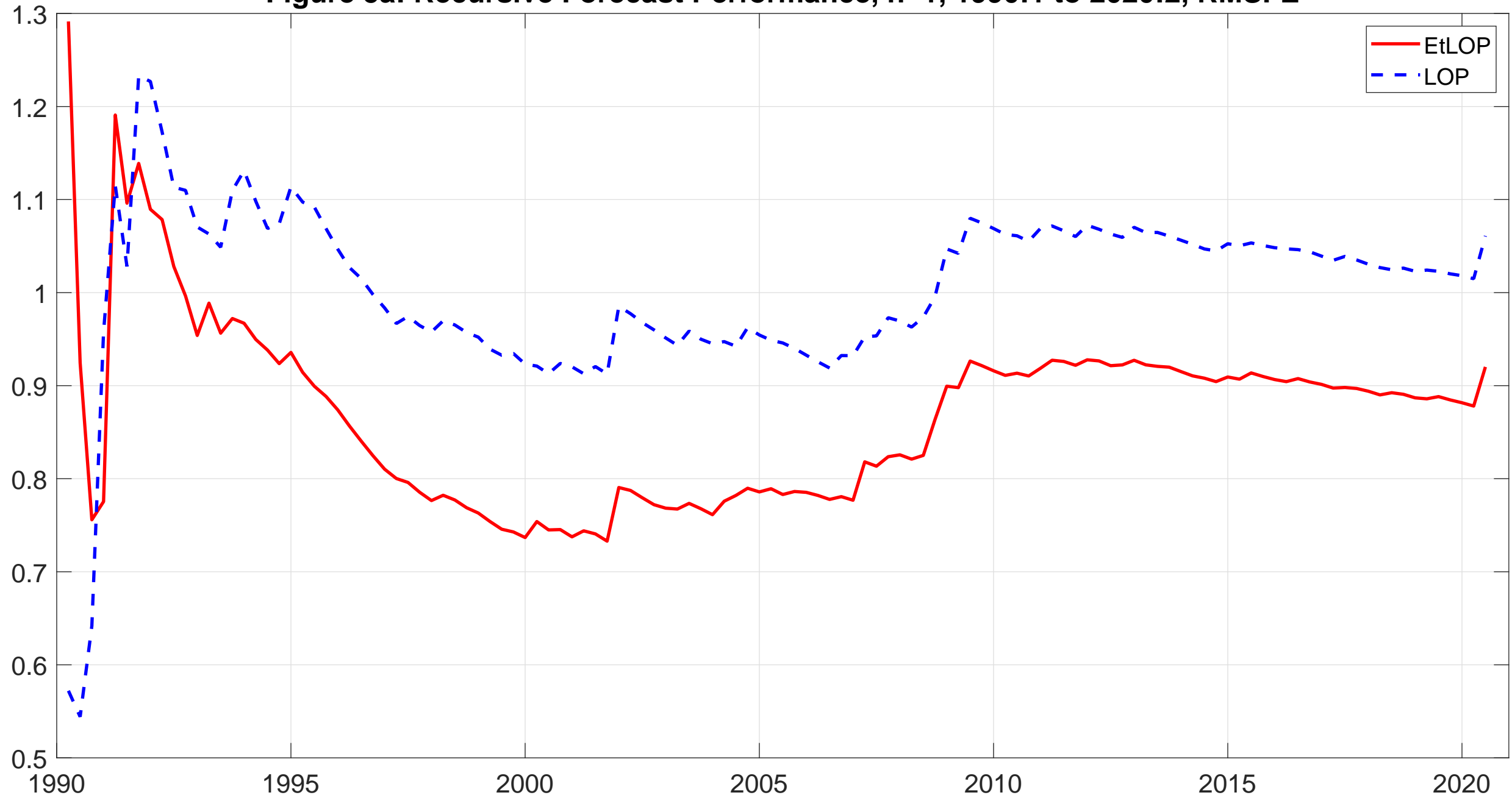
Figure 5a: Recursive Forecast Performance, h=1, 1990:1 to 2020:2, RMSFE
