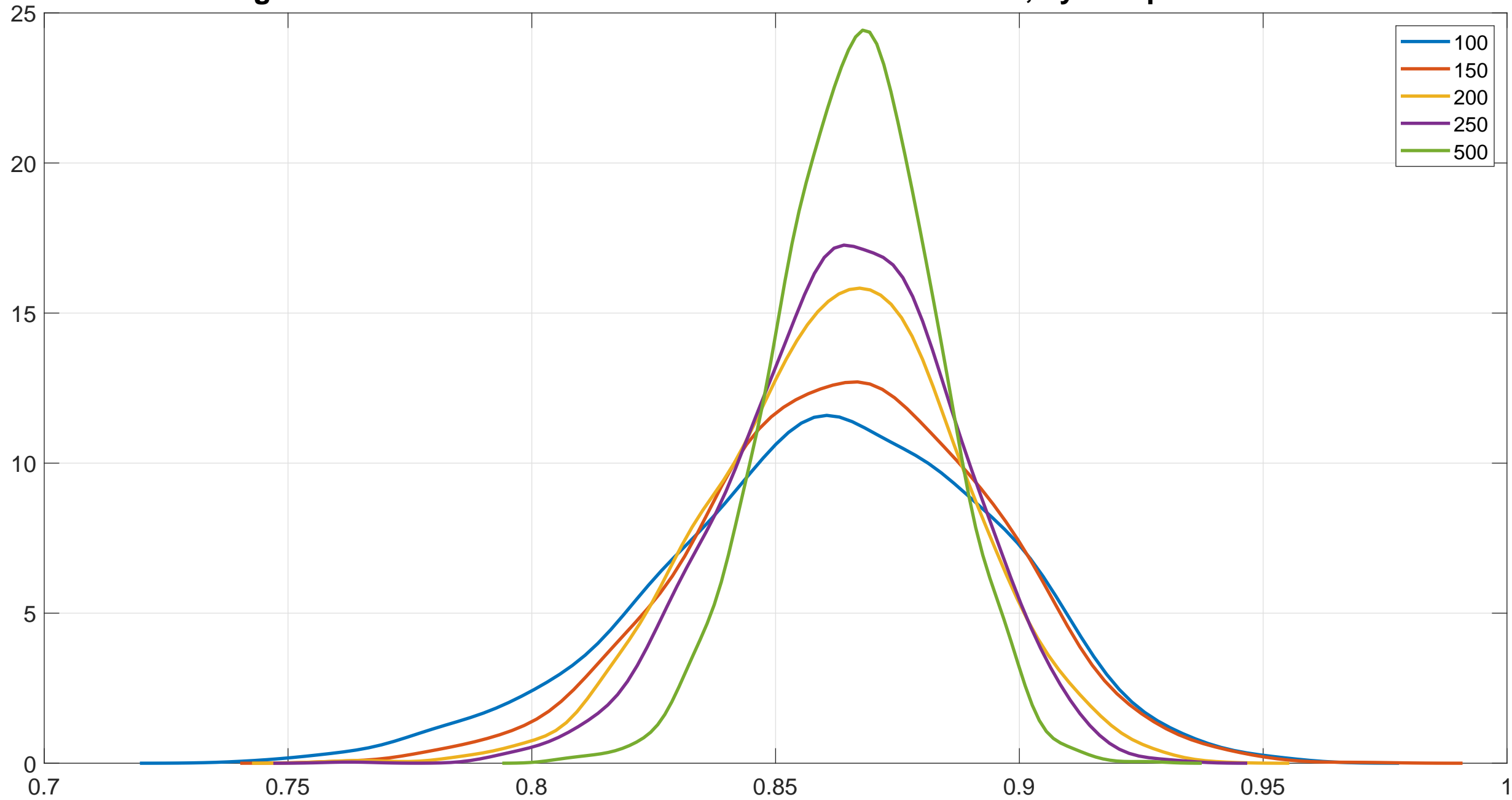
Figure 3: EtLOPs Relative CRPS Performance Simulation, by Sample Size
