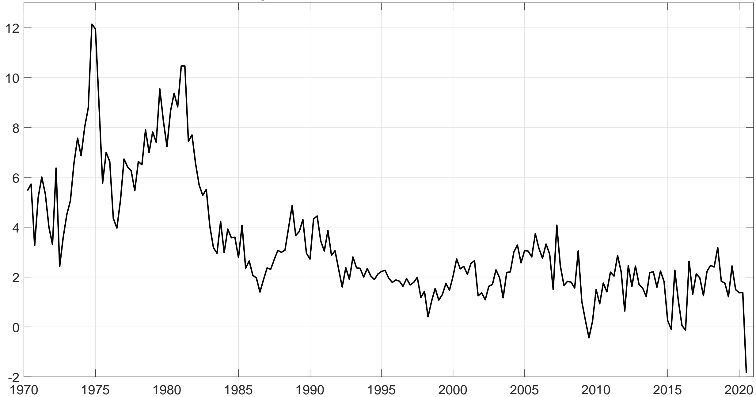
Figure 4a: U.S. Inflation, 1970:1 to 2020:2
