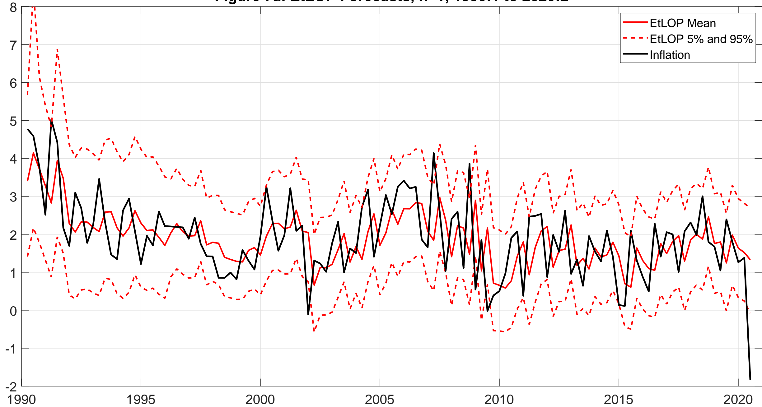
Figure 7a: EtLOP Forecasts, h=1, 1990:1 to 2020:2
