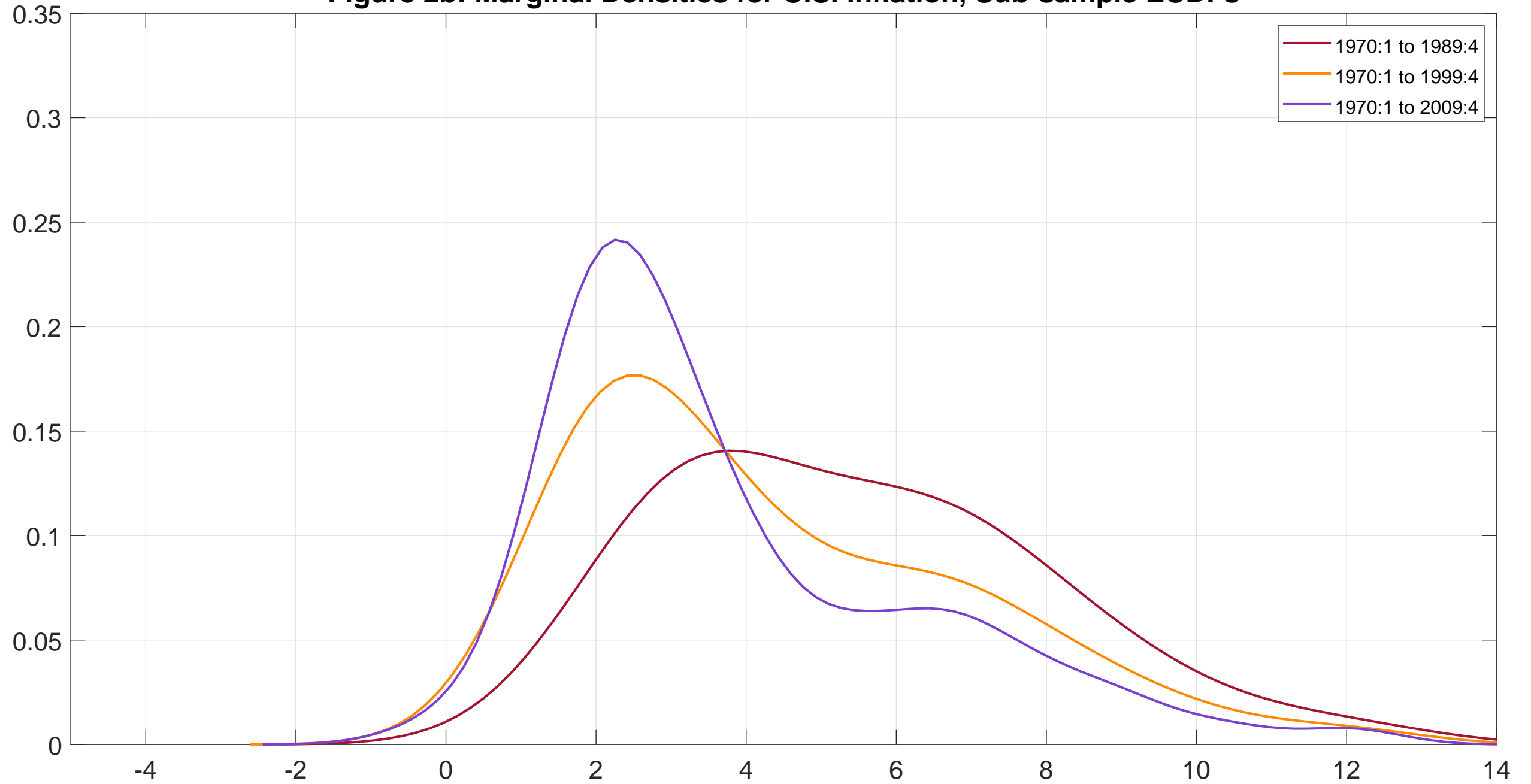
Figure 2b: Marginal Densities for U.S. Inflation, Sub-sample ECDFs
