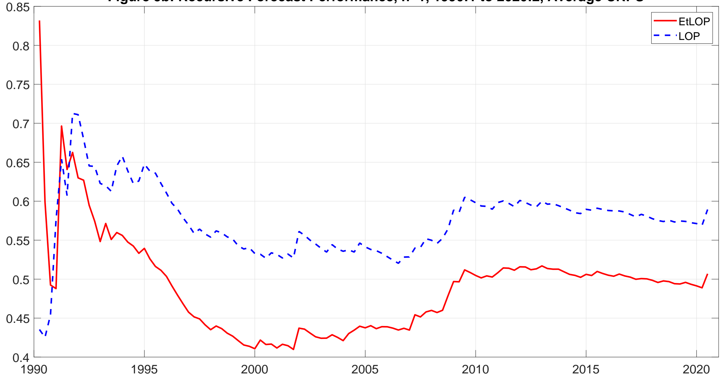
Figure 5b: Recursive Forecast Performance, h=1, 1990:1 to 2020:2, Average CRPS
