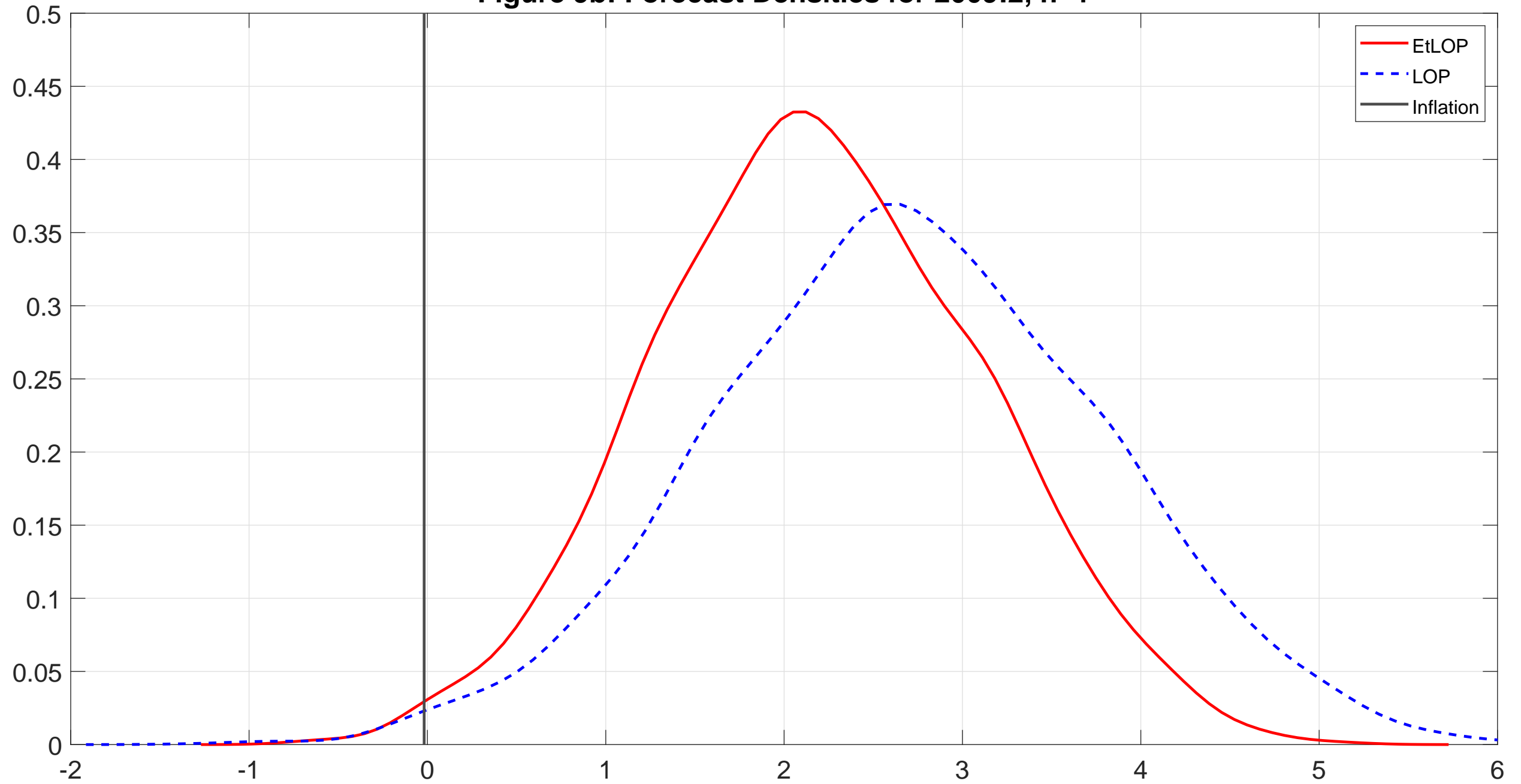
Figure 9b: Forecast Densities for 2009:2, h=1
