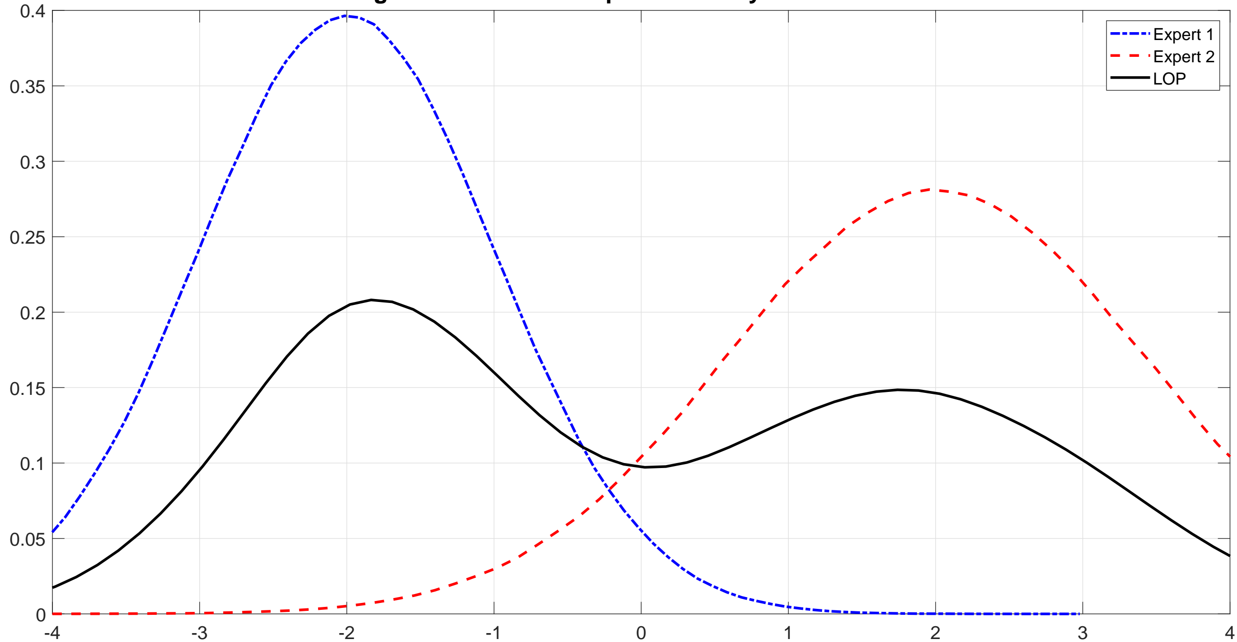
Figure 1a: LOP and Experts' Density Forecasts
