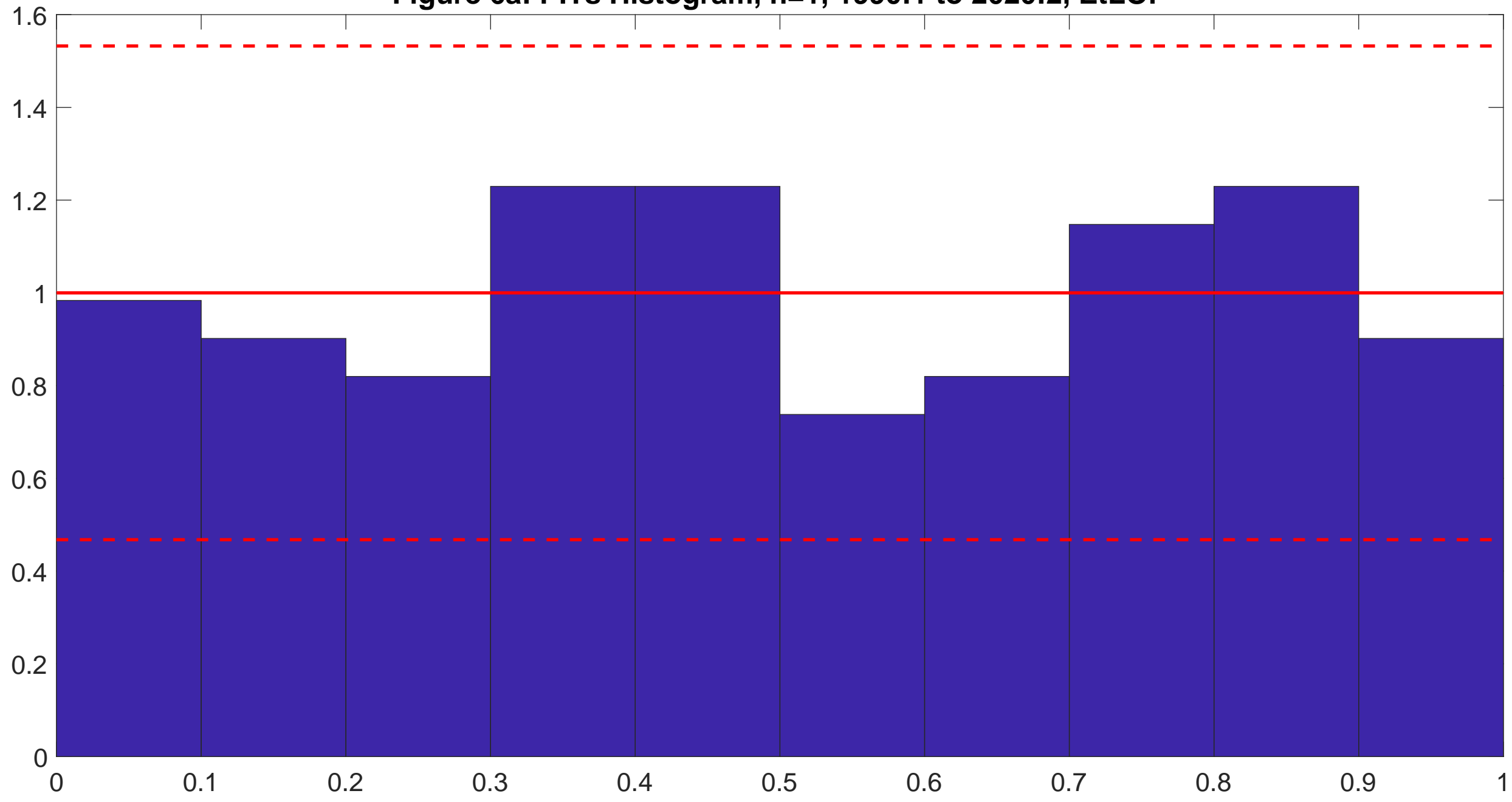
Figure 6a: PITs Histogram, h=1, 1990:1 to 2020:2, EtLOP
