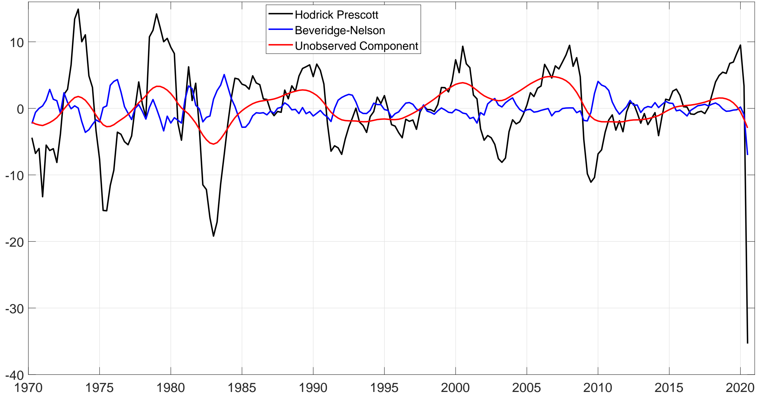
Figure 4c: U.S. Output Gaps, 1970:1 to 2020
