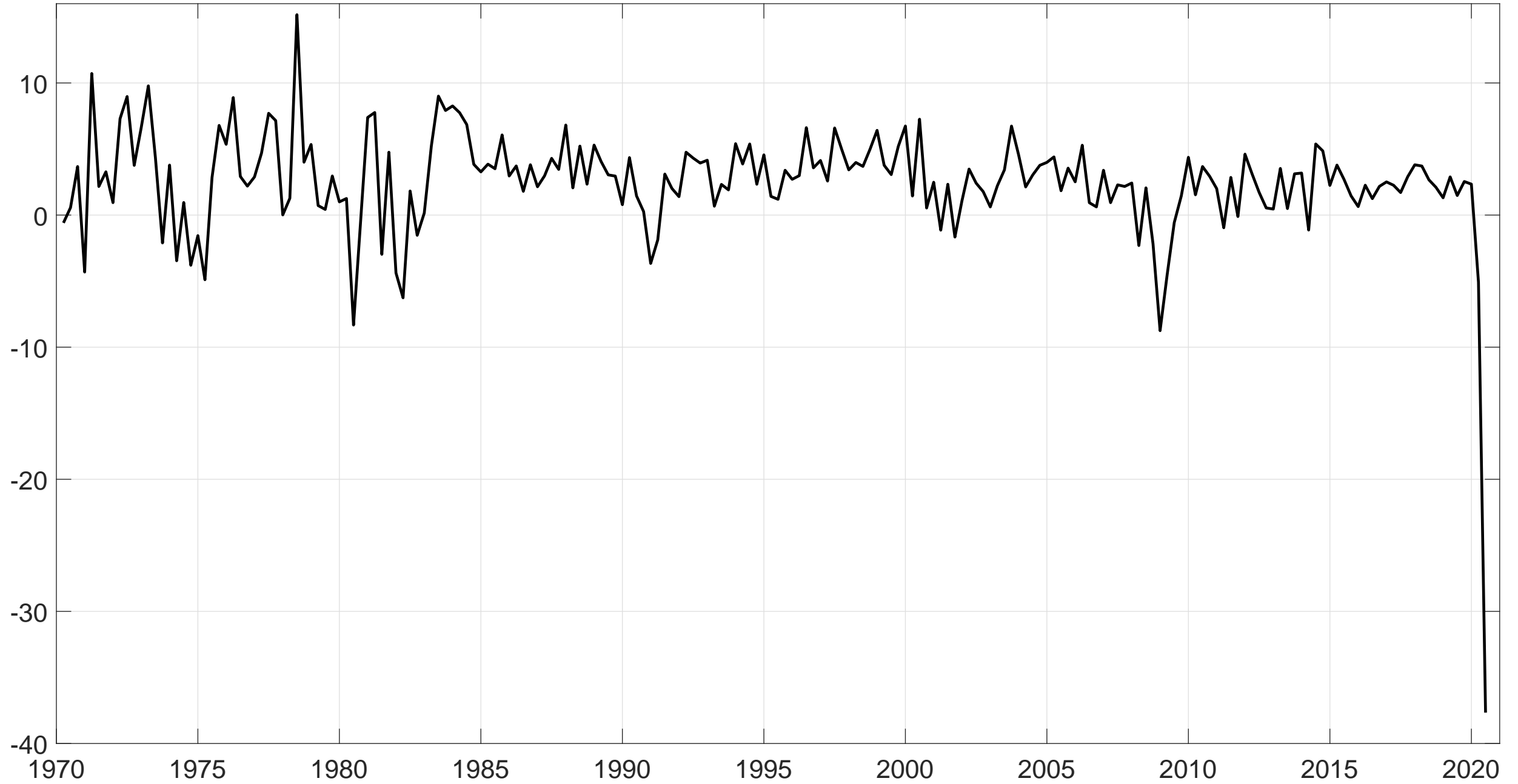
Figure 4b: U.S. Real Output Growth, 1970:1 to 2020
