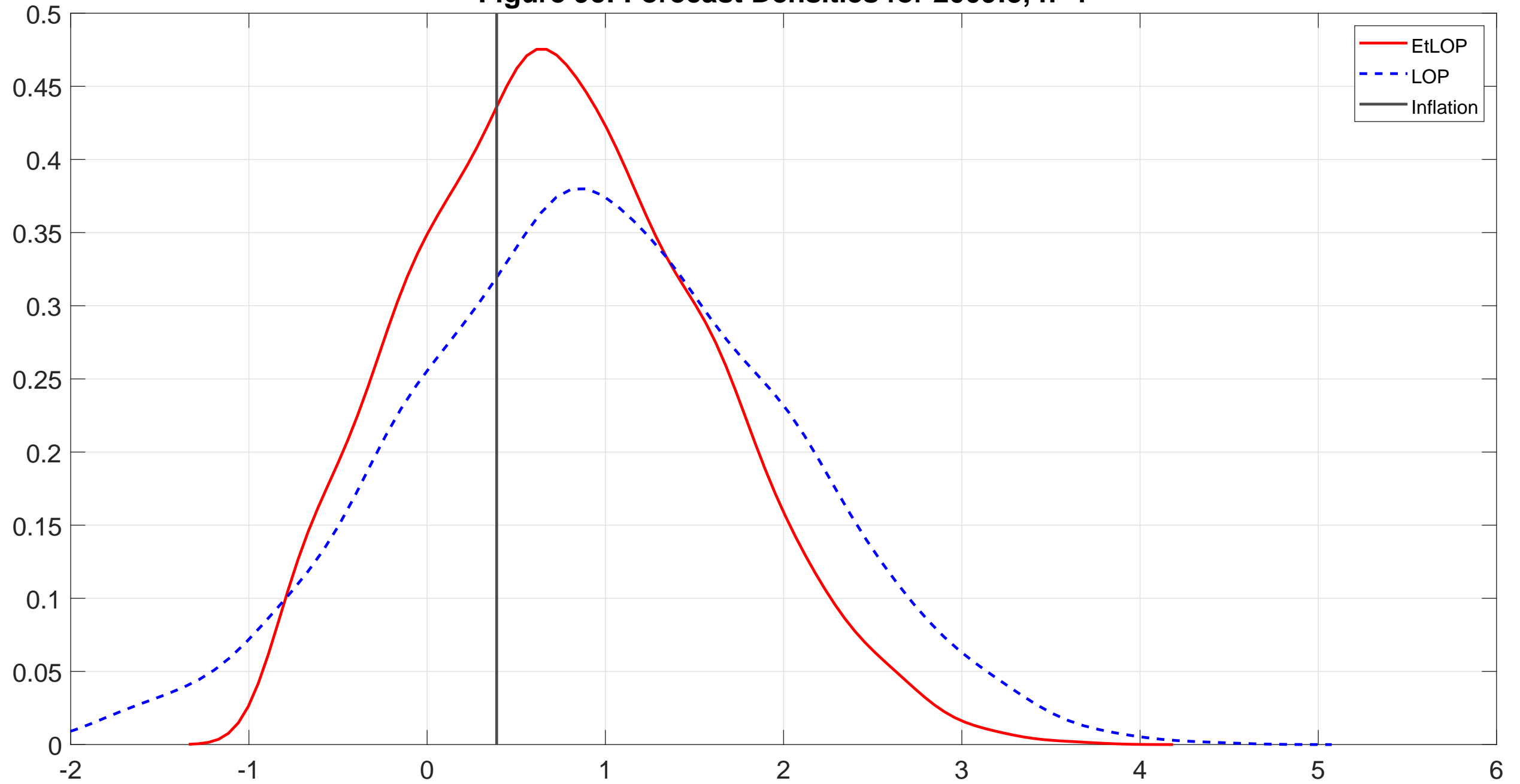
Figure 9c: Forecast Densities for 2009:3, h=1
