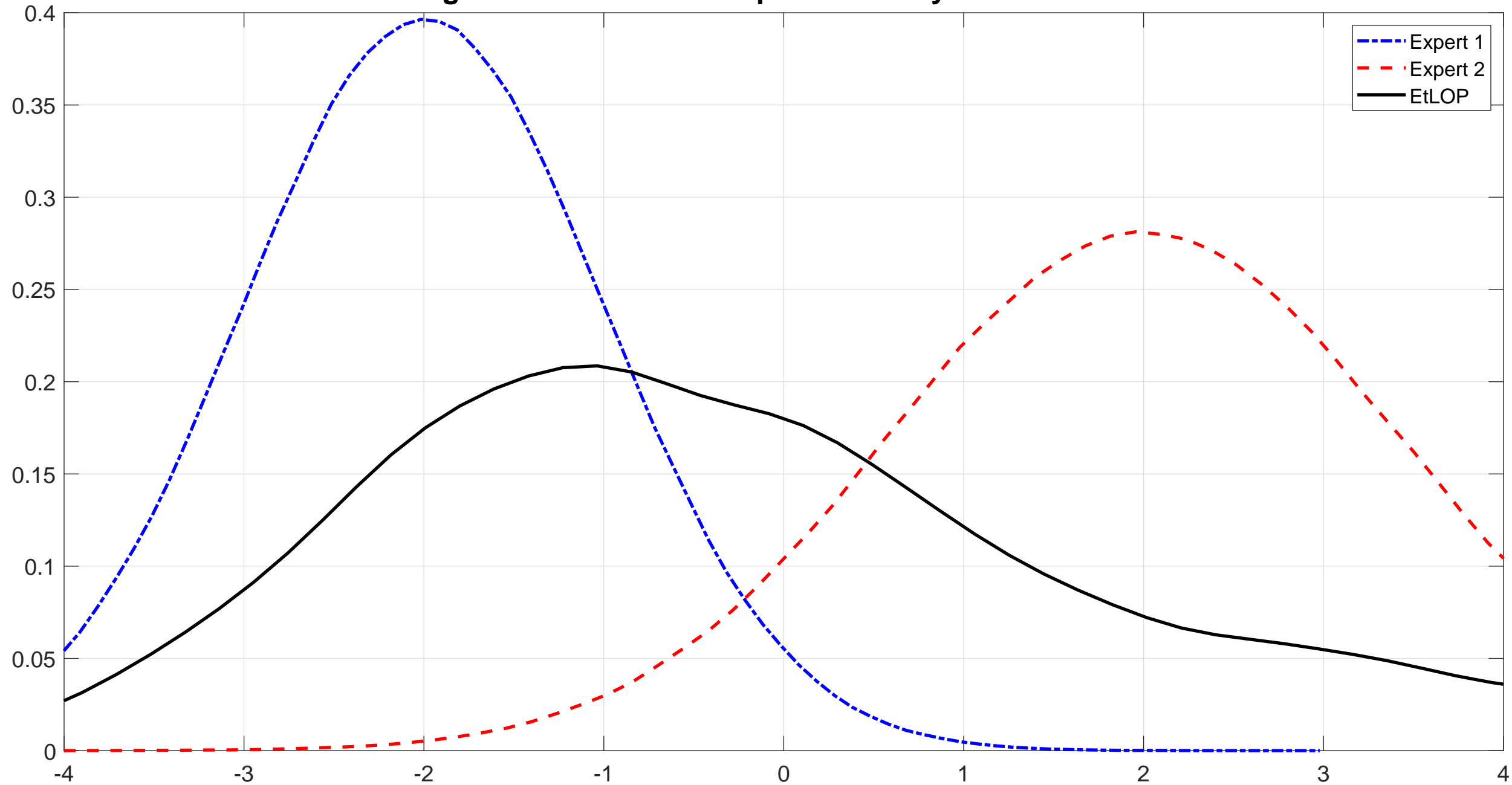
Figure 1b: EtLOP and Experts' Density Forecasts
