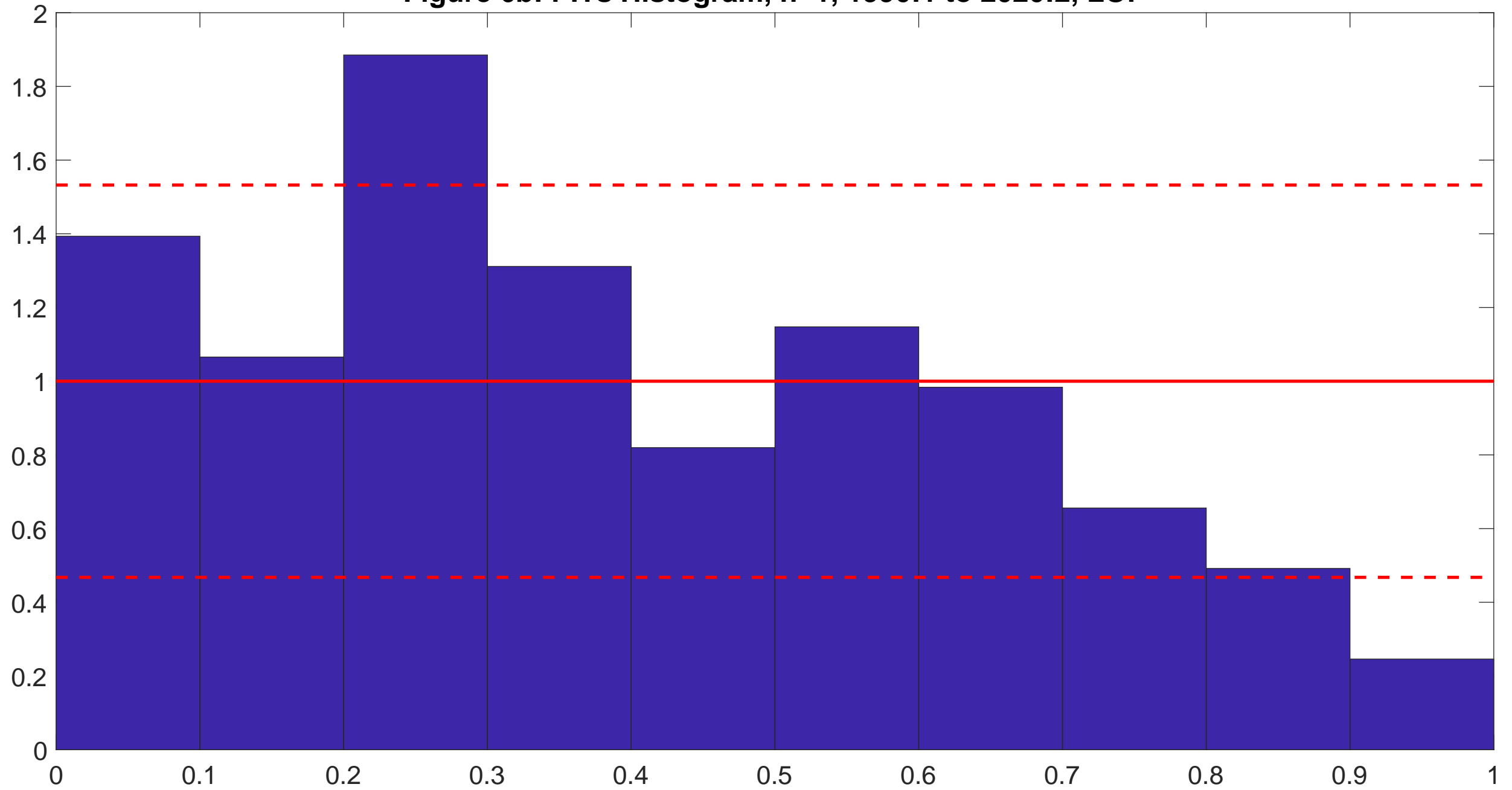
Figure 6b: PITs Histogram, h=1, 1990:1 to 2020:2, LOP
