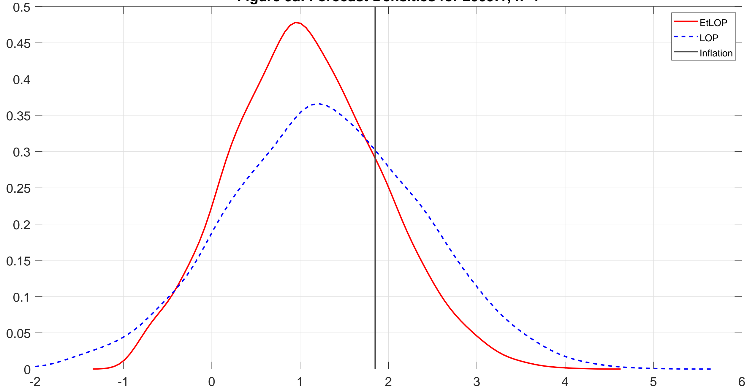
Figure 9a: Forecast Densities for 2009:1, h=1
