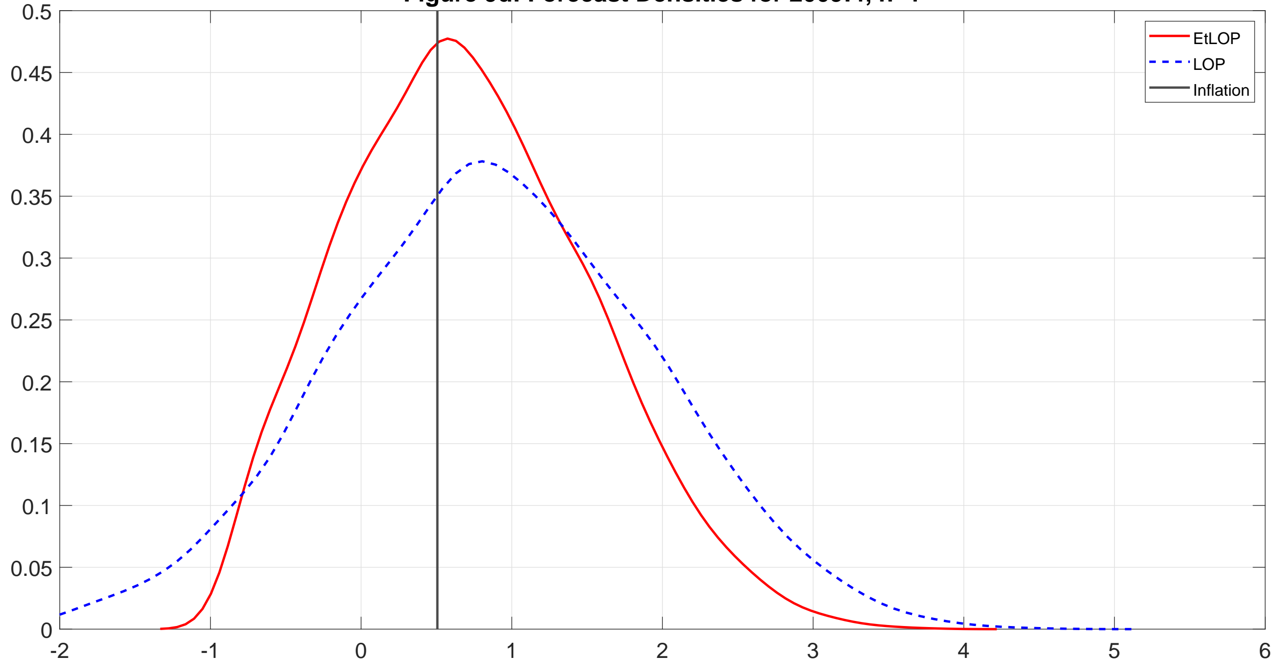
Figure 9d: Forecast Densities for 2009:4, h=1
