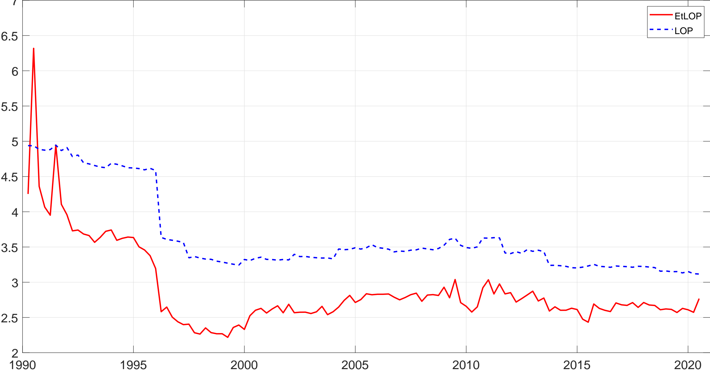
Figure 8a: Uncertainty Range (95%-5%)
