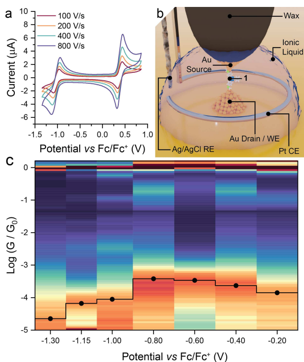
Figure 3. Electrochemical Experiments. a) Cyclic voltammetry of 1 in degassed \text{CH}_2\text{Cl}_2 , with 0.1 M tetrabutylammonium hexafluorophosphate as supporting electrolyte. Potentials referenced to the ferrocene/ferrocenium redox couple using a decamethylferrocene standard. b) Depiction of the 4-electrode setup used in the single-molecule electrochemical gating studies with the molecular junction in place. c) Heatmap (blue = low counts; red = high counts) of electrochemically-gated single-molecule conductance data (compiled with 10 bins per decade from more than 5500 individual scans at each potential) across the electrochemical window explored in the ionic liquid 1-butyl-3-methylimidazolium triflate, with points indicating the most probable conductance determined from a Gaussian fit of the conductance histogram at each potential overlaid in black. Potential referenced to the ferrocene/ferrocenium redox couple as internal standard.
