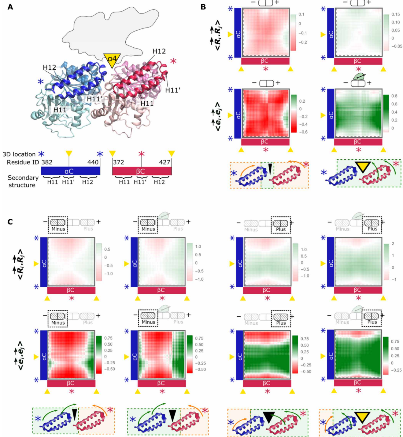
Fig. 4. Response of the outer surface of MT to Kin1 binding. (A) Top: Side view of a tubulin dimer with C-terminal domains of \alpha - and \beta -tubulins ( \alpha C and \beta C , highlighted with darkest blue and red colors), consisting of H11, H11', and H12 helices (35). Upon binding, helix \alpha 4 in Kin1 (shown as a yellow triangle) is between the two C-terminal domains and at the intradimer interface cleft. Bottom: Sequences of \alpha C and \beta C are represented as blue and red bars, respectively. The locations of the residues near the intradimer and interdimer interfaces are marked with yellow triangles and stars, corresponding to the top figure. (B) Plots of \langle \vec{R}_i \cdot \vec{R}_j \rangle (top) and \langle \vec{e}_i \cdot \vec{e}_j \rangle (center) between C-terminal domains of an \alpha\beta -tubulin dimer in the absence of Kin1 (left) and with the bound trailing head (right). The plots are on the same color scale with green (red) representing positive (negative) values. Bottom: The positions of the residues with positive correlations are mapped to side views of corresponding C-terminal domains with dashed green boxes; the negative correlations are in orange boxes. (C) Similar to (B) but correlation matrices are calculated for minus- and plus-end tubulin dimers in the (Short) 1 -D-Near construct.
