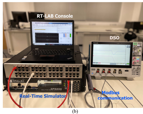
Fig. 19. The second experimental validation (a)Two-area interconnected power system in RT-LAB (b) The OPAL-RT experimental test.
