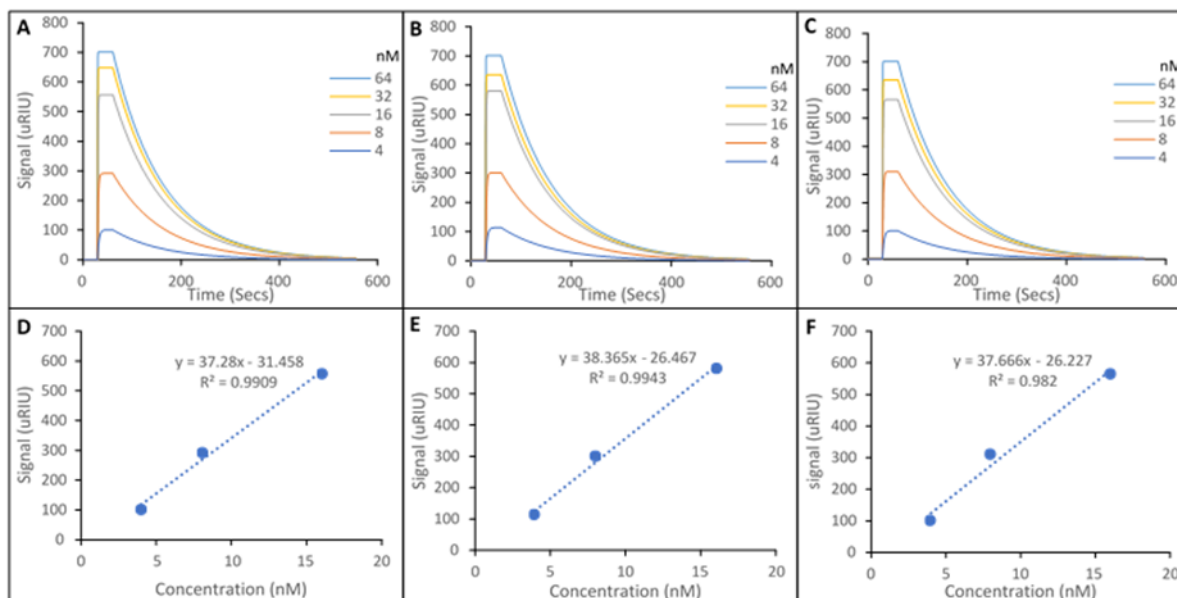
Figure 3: Representative SPR curves showing rebinding of target and non-target SARMs to the immobilised nanoMIPs. Five concentrations of analyte in FBS. (A) Andarine binding to Andarine-imprinted nanoMIPs; (B) Ligandrol binding to Ligandrol-imprinted nanoMIPs; (C) RAD-140 binding to RAD-140-imprinted nanoMIPs: Elucidation of limit of detection for SPE sensor. Relative signal vs concentration (D) Andarine binding to Andarine-imprinted nanoMIPs concentration calibration; (E) Ligandrol binding to Ligandrol-imprinted nanoMIPs concentration calibration; (F) RAD-140 binding to RAD-140-imprinted nanoMIPs concentration calibration.
